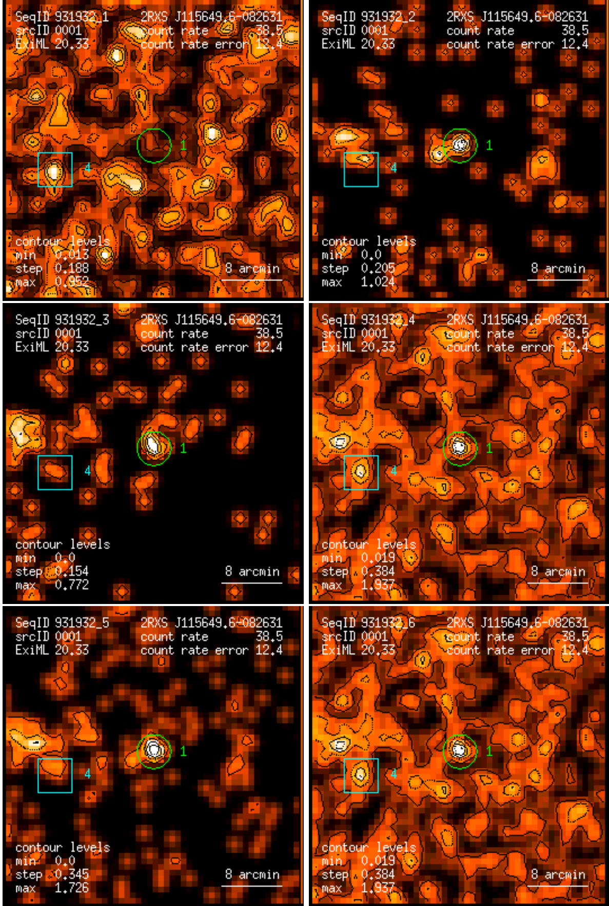
Figure 1: RASS 931932: detection 0001: band rate images, Gaussian filter: (1) PSPC channels 11 – 41, (2) 52 – 90, (3) 91 – 201, (4) 11 – 235, (5) 52 – 201, (6) 11 – 201. Broad band rates in counts/ks. Band rate contour levels in counts/ks/arcmin 2 .
