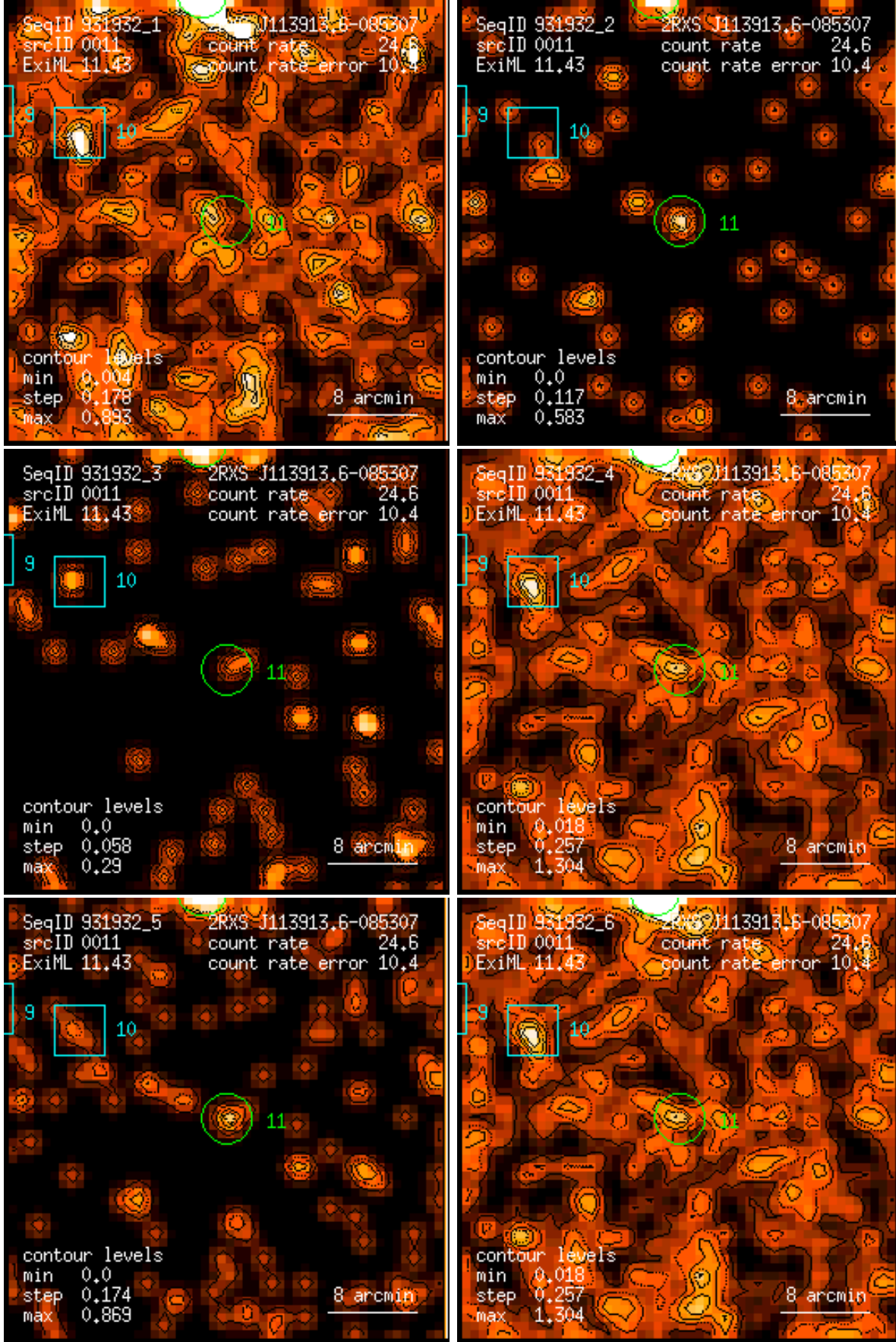
Figure 11: RASS 931932: detection 0011: band rate images, Gaussian filter: (1) PSPC channels 11 – 41, (2) 52 – 90, (3) 91 – 201, (4) 11 – 235, (5) 52 – 201, (6) 11 – 201. Broad band rates in counts/ks. Band rate contour levels in counts/ks/arcmin 2 .
