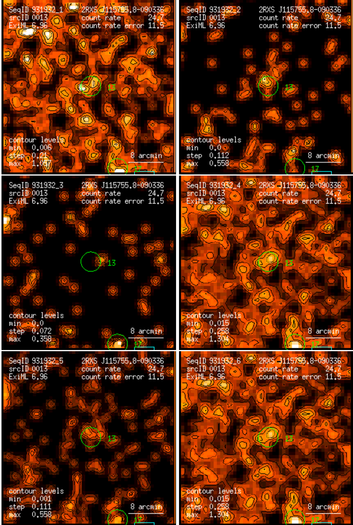
Figure 13: RASS 931932: detection 0013: band rate images, Gaussian filter: (1) PSPC channels 11 – 41, (2) 52 – 90, (3) 91 – 201, (4) 11 – 235, (5) 52 – 201, (6) 11 – 201. Broad band rates in counts/ks. Band rate contour levels in counts/ks/arcmin 2 .
