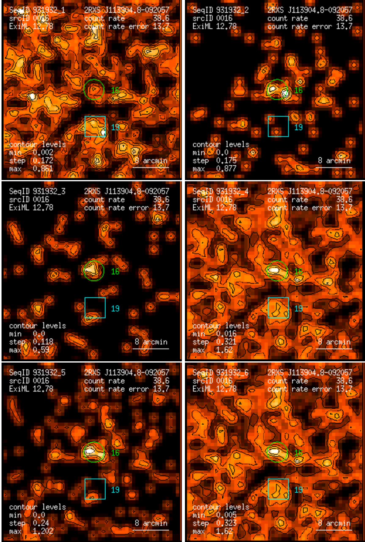
Figure 16: RASS 931932: detection 0016: band rate images, Gaussian filter: (1) PSPC channels 11 – 41, (2) 52 – 90, (3) 91 – 201, (4) 11 – 235, (5) 52 – 201, (6) 11 – 201. Broad band rates in counts/ks. Band rate contour levels in counts/ks/arcmin 2 .
