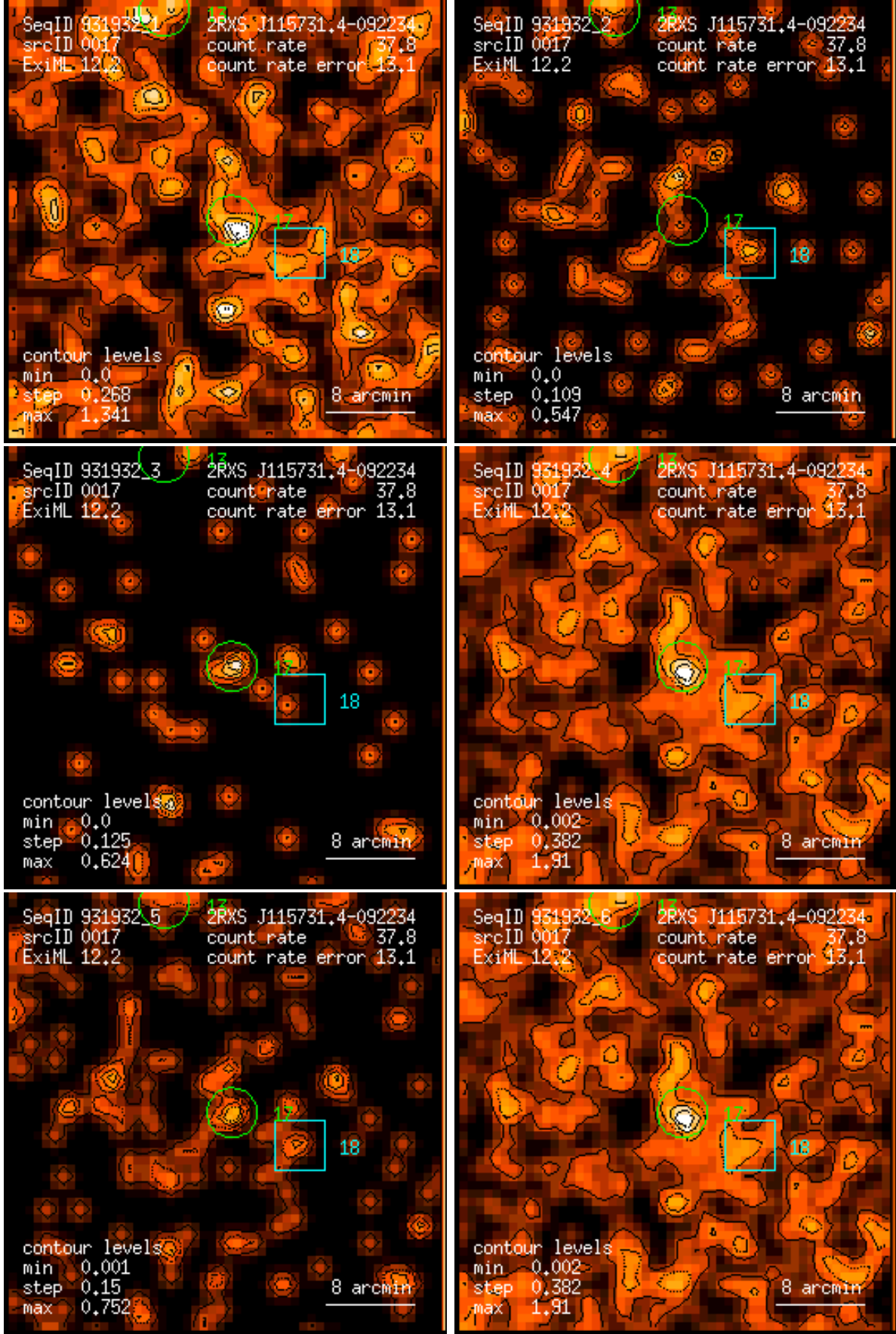
Figure 17: RASS 931932: detection 0017: band rate images, Gaussian filter: (1) PSPC channels 11 – 41, (2) 52 – 90, (3) 91 – 201, (4) 11 – 235, (5) 52 – 201, (6) 11 – 201. Broad band rates in counts/ks. Band rate contour levels in counts/ks/arcmin 2 .
