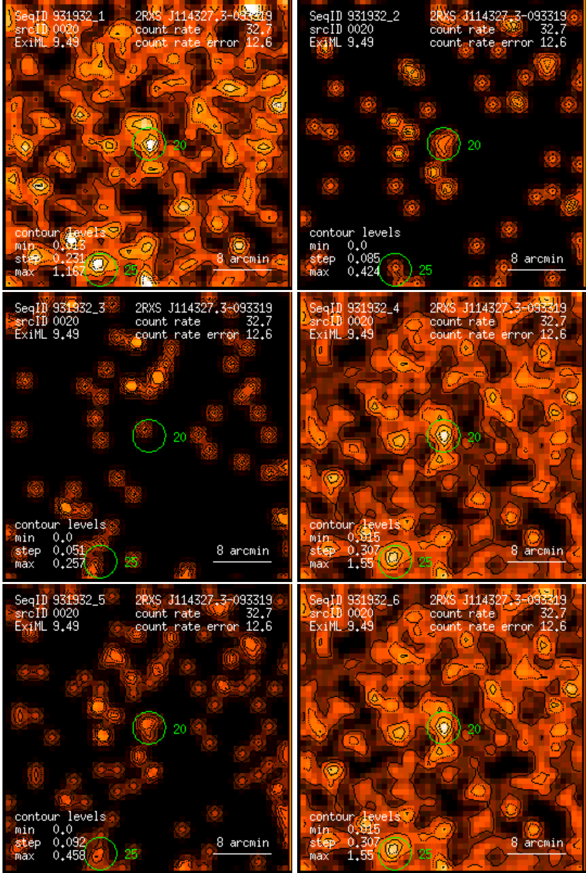
Figure 20: RASS 931932: detection 0020: band rate images, Gaussian filter: (1) PSPC channels 11 – 41, (2) 52 – 90, (3) 91 – 201, (4) 11 – 235, (5) 52 – 201, (6) 11 – 201. Broad band rates in counts/ks. Band rate contour levels in counts/ks/arcmin 2 .
