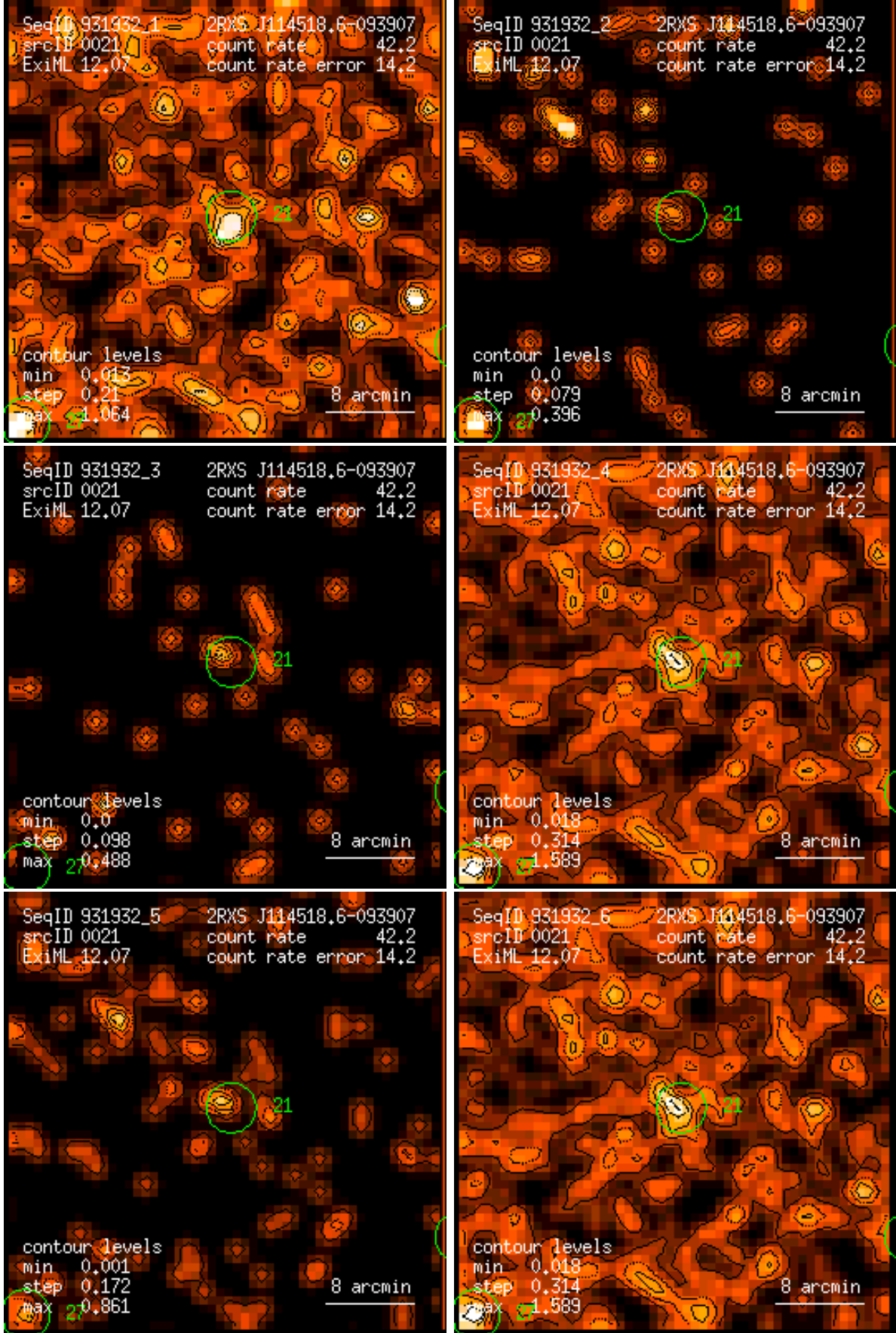
Figure 21: RASS 931932: detection 0021: band rate images, Gaussian filter: (1) PSPC channels 11 – 41, (2) 52 – 90, (3) 91 – 201, (4) 11 – 235, (5) 52 – 201, (6) 11 – 201. Broad band rates in counts/ks. Band rate contour levels in counts/ks/arcmin 2 .
