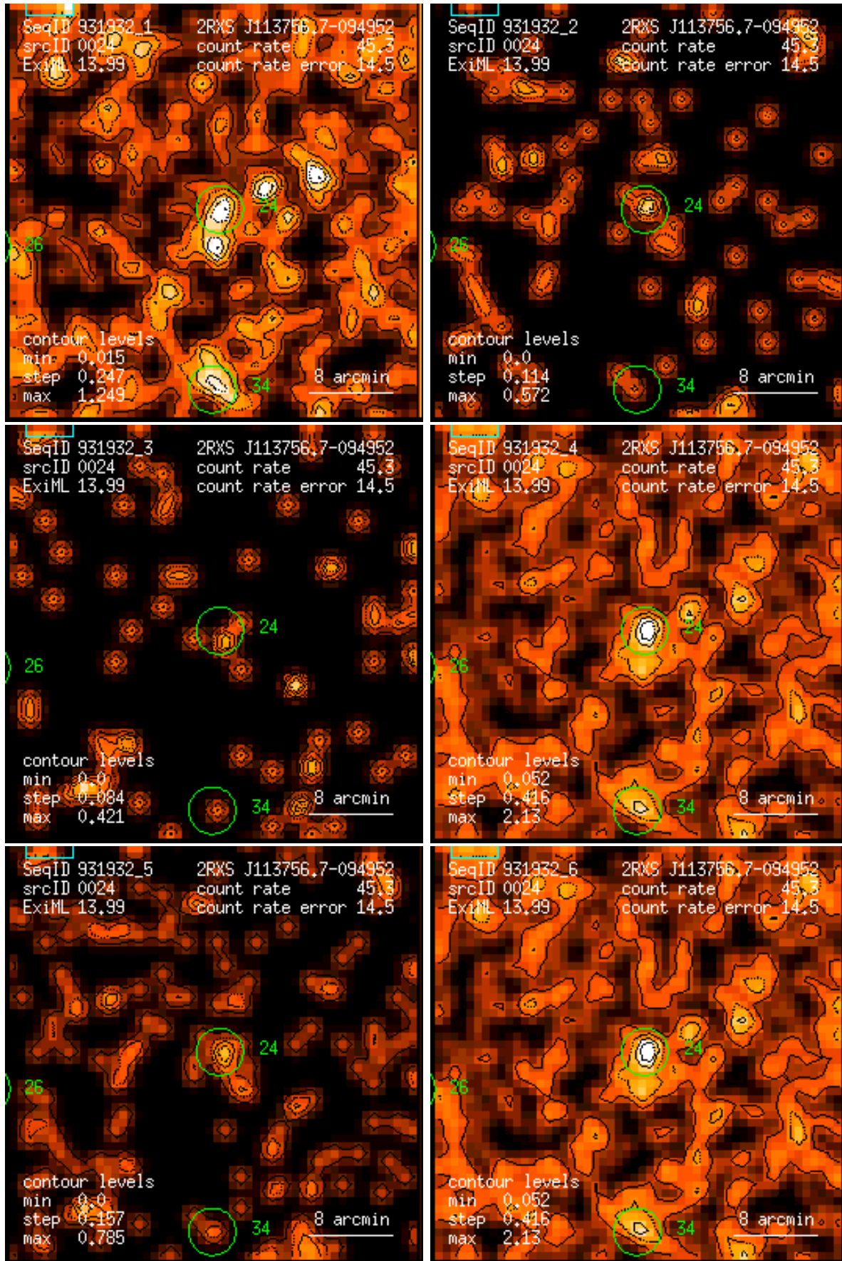
Figure 24: RASS 931932: detection 0024: band rate images, Gaussian filter: (1) PSPC channels 11 – 41, (2) 52 – 90, (3) 91 – 201, (4) 11 – 235, (5) 52 – 201, (6) 11 – 201. Broad band rates in counts/ks. Band rate contour levels in counts/ks/arcmin 2 .
