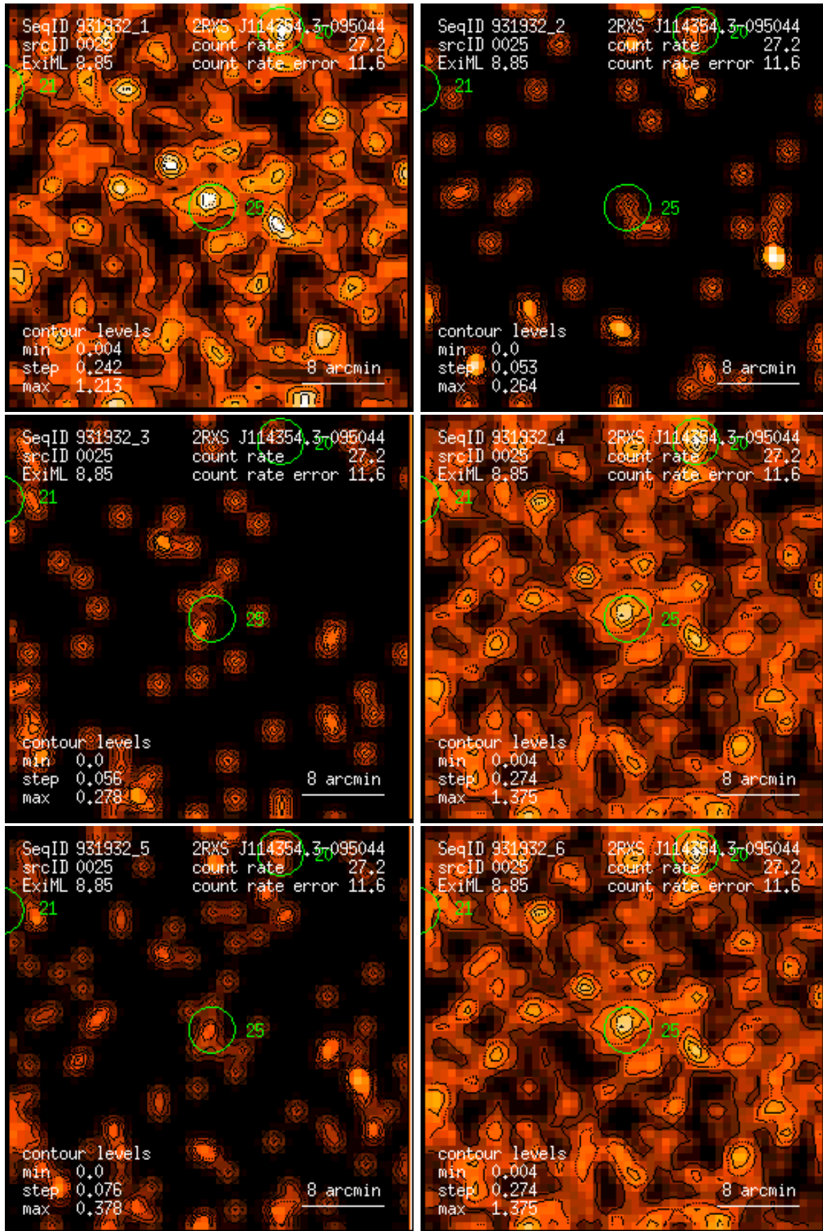
Figure 25: RASS 931932: detection 0025: band rate images, Gaussian filter: (1) PSPC channels 11 – 41, (2) 52 – 90, (3) 91 – 201, (4) 11 – 235, (5) 52 – 201, (6) 11 – 201. Broad band rates in counts/ks. Band rate contour levels in counts/ks/arcmin 2 .
