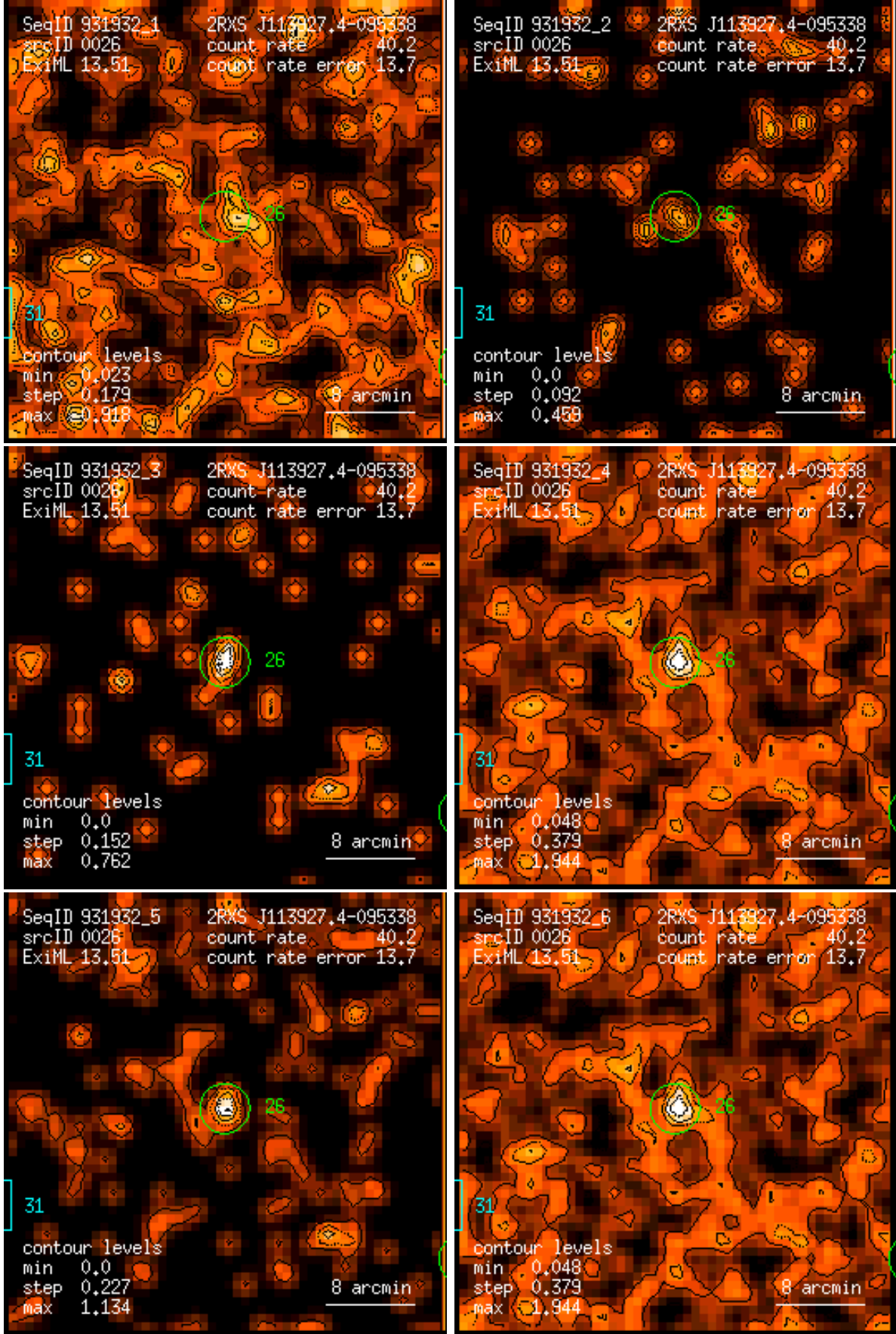
Figure 26: RASS 931932: detection 0026: band rate images, Gaussian filter: (1) PSPC channels 11 – 41, (2) 52 – 90, (3) 91 – 201, (4) 11 – 235, (5) 52 – 201, (6) 11 – 201. Broad band rates in counts/ks. Band rate contour levels in counts/ks/arcmin 2 .
