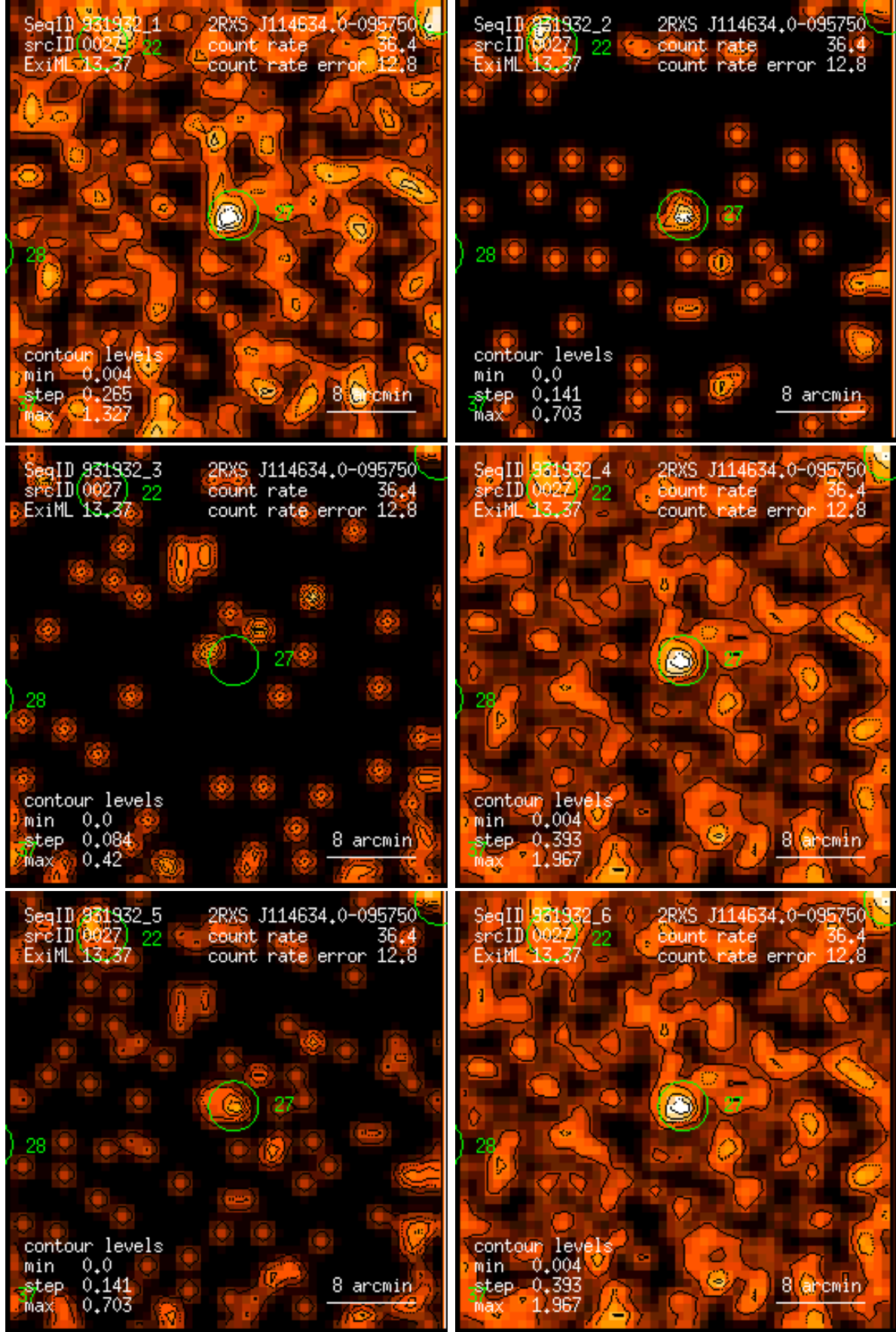
Figure 27: RASS 931932: detection 0027: band rate images, Gaussian filter: (1) PSPC channels 11 – 41, (2) 52 – 90, (3) 91 – 201, (4) 11 – 235, (5) 52 – 201, (6) 11 – 201. Broad band rates in counts/ks. Band rate contour levels in counts/ks/arcmin 2 .
