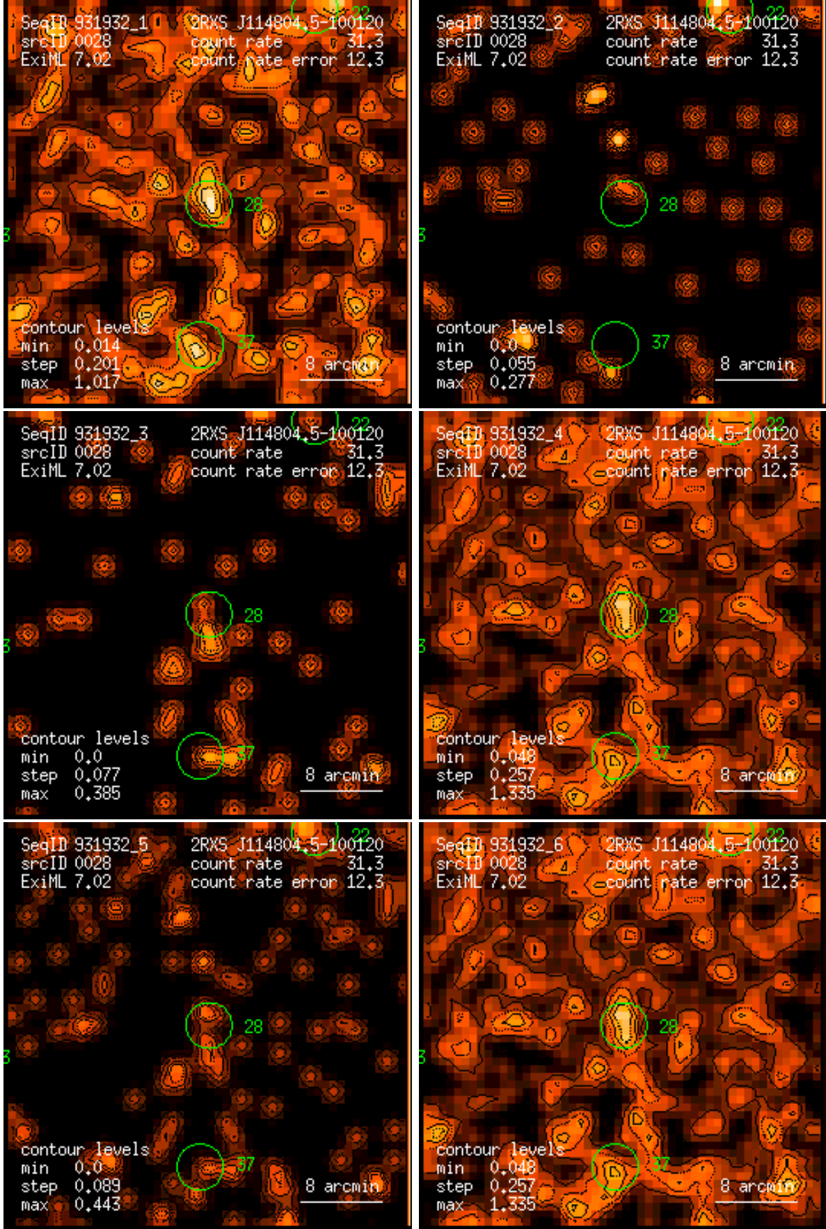
Figure 28: RASS 931932: detection 0028: band rate images, Gaussian filter: (1) PSPC channels 11 – 41, (2) 52 – 90, (3) 91 – 201, (4) 11 – 235, (5) 52 – 201, (6) 11 – 201. Broad band rates in counts/ks. Band rate contour levels in counts/ks/arcmin 2 .
