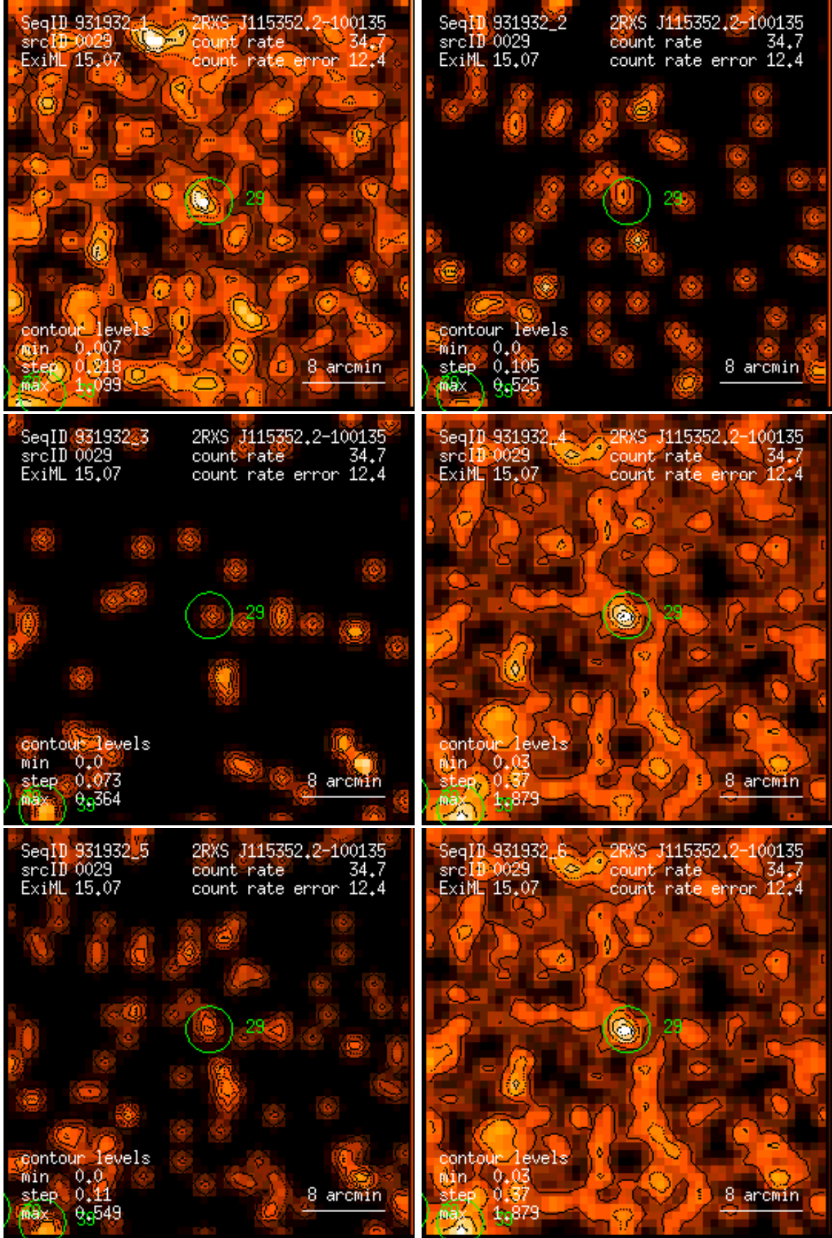
Figure 29: RASS 931932: detection 0029: band rate images, Gaussian filter: (1) PSPC channels 11 – 41, (2) 52 – 90, (3) 91 – 201, (4) 11 – 235, (5) 52 – 201, (6) 11 – 201. Broad band rates in counts/ks. Band rate contour levels in counts/ks/arcmin 2 .
