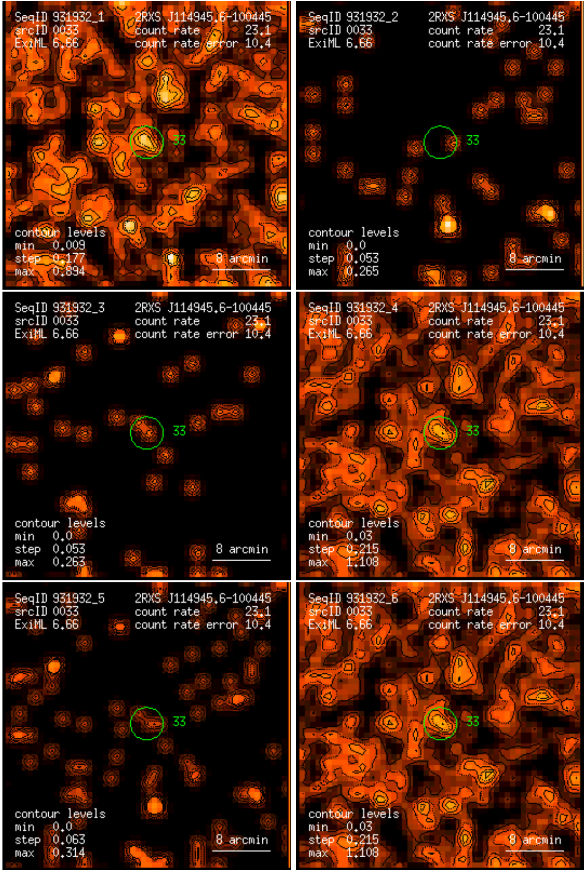
Figure 33: RASS 931932: detection 0033: band rate images, Gaussian filter: (1) PSPC channels 11 – 41, (2) 52 – 90, (3) 91 – 201, (4) 11 – 235, (5) 52 – 201, (6) 11 – 201. Broad band rates in counts/ks. Band rate contour levels in counts/ks/arcmin 2 .
