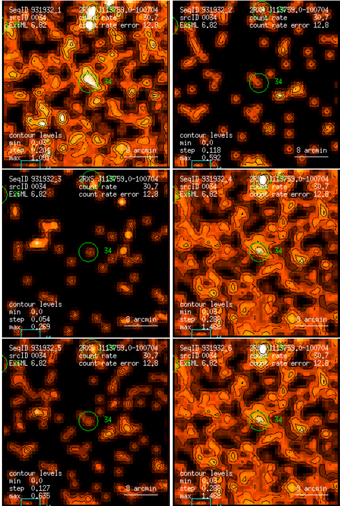
Figure 34: RASS 931932: detection 0034: band rate images, Gaussian filter: (1) PSPC channels 11 – 41, (2) 52 – 90, (3) 91 – 201, (4) 11 – 235, (5) 52 – 201, (6) 11 – 201. Broad band rates in counts/ks. Band rate contour levels in counts/ks/arcmin 2 .
