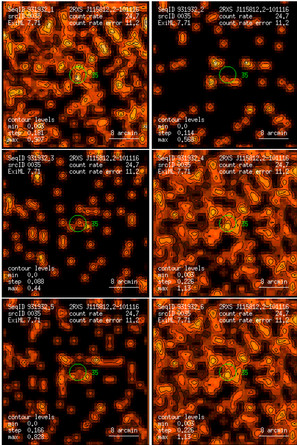
Figure 35: RASS 931932: detection 0035: band rate images, Gaussian filter: (1) PSPC channels 11 – 41, (2) 52 – 90, (3) 91 – 201, (4) 11 – 235, (5) 52 – 201, (6) 11 – 201. Broad band rates in counts/ks. Band rate contour levels in counts/ks/arcmin 2 .
