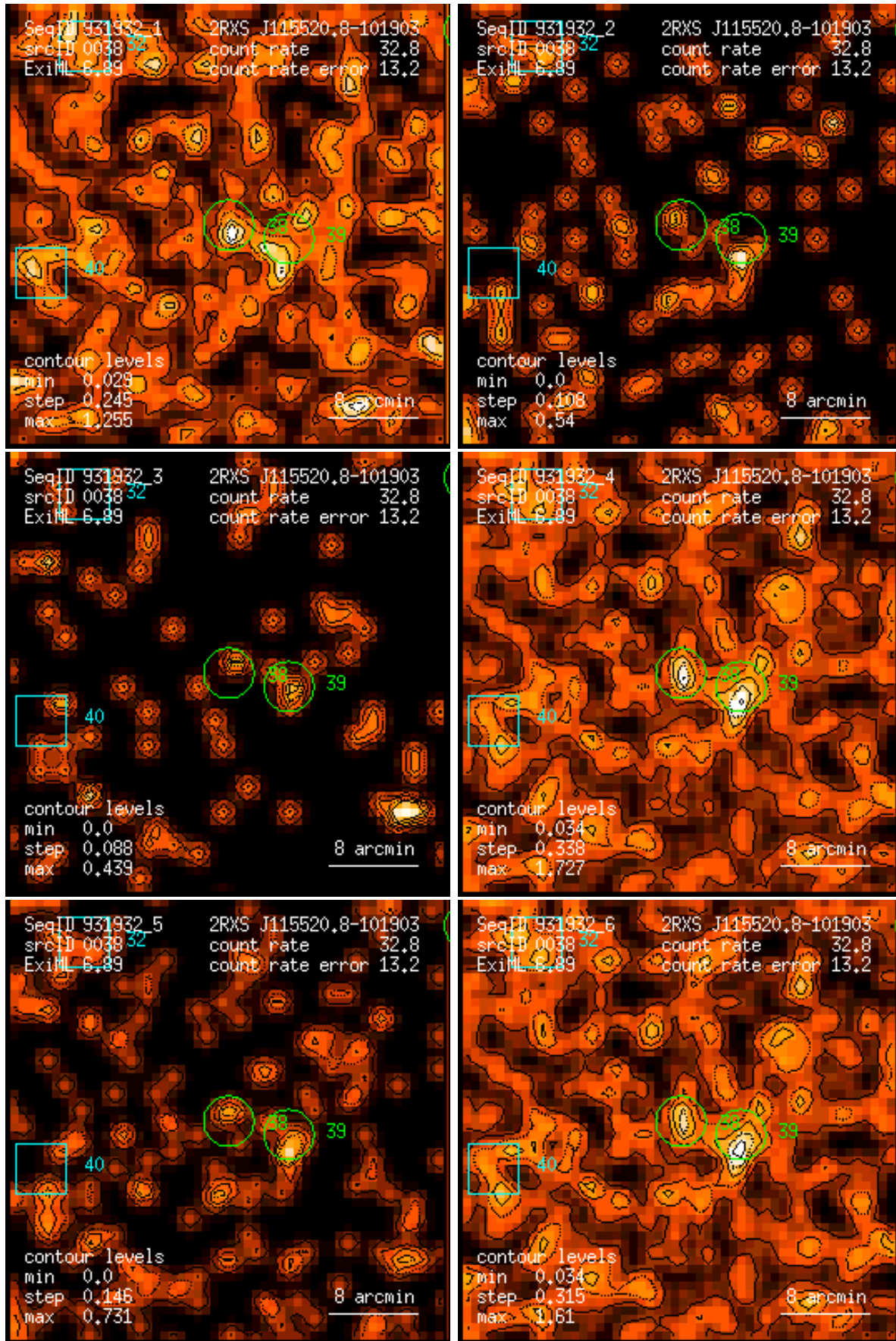
Figure 38: RASS 931932: detection 0038: band rate images, Gaussian filter: (1) PSPC channels 11 – 41, (2) 52 – 90, (3) 91 – 201, (4) 11 – 235, (5) 52 – 201, (6) 11 – 201. Broad band rates in counts/ks. Band rate contour levels in counts/ks/arcmin 2 .
