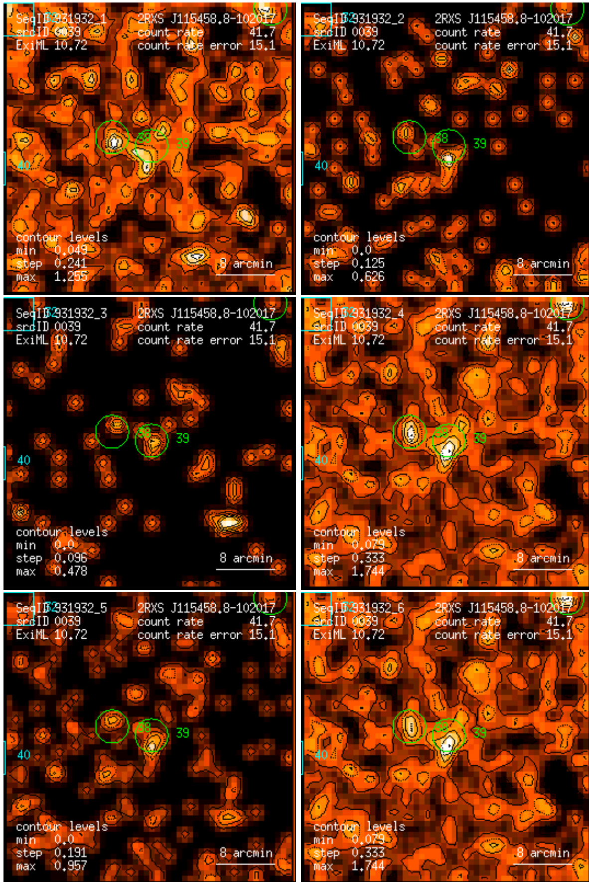
Figure 39: RASS 931932: detection 0039: band rate images, Gaussian filter: (1) PSPC channels 11 – 41, (2) 52 – 90, (3) 91 – 201, (4) 11 – 235, (5) 52 – 201, (6) 11 – 201. Broad band rates in counts/ks. Band rate contour levels in counts/ks/arcmin 2 .
