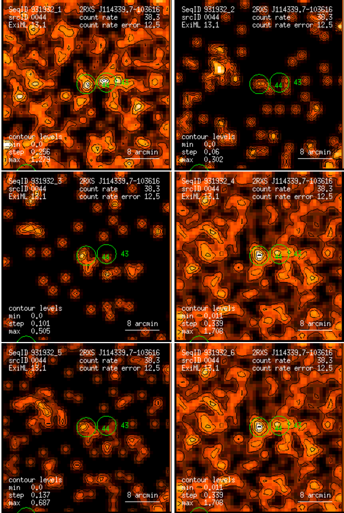
Figure 44: RASS 931932: detection 0044: band rate images, Gaussian filter: (1) PSPC channels 11 – 41, (2) 52 – 90, (3) 91 – 201, (4) 11 – 235, (5) 52 – 201, (6) 11 – 201. Broad band rates in counts/ks. Band rate contour levels in counts/ks/arcmin 2 .
