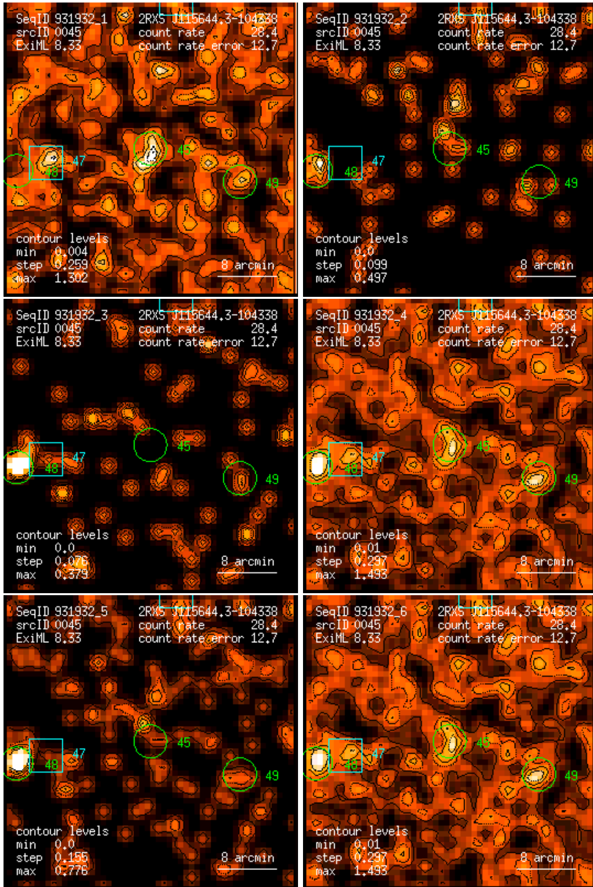
Figure 45: RASS 931932: detection 0045: band rate images, Gaussian filter: (1) PSPC channels 11 – 41, (2) 52 – 90, (3) 91 – 201, (4) 11 – 235, (5) 52 – 201, (6) 11 – 201. Broad band rates in counts/ks. Band rate contour levels in counts/ks/arcmin 2 .
