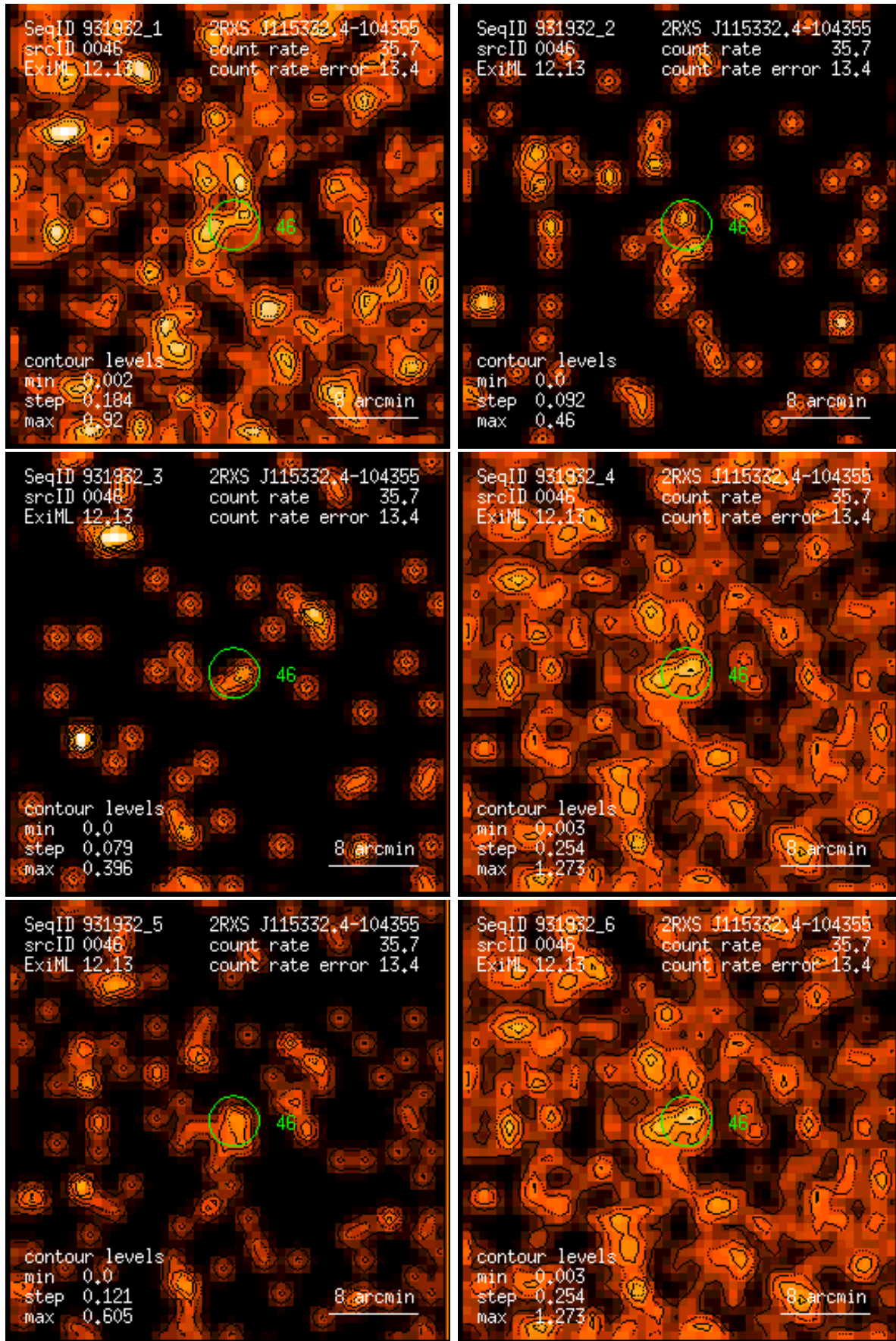
Figure 46: RASS 931932: detection 0046: band rate images, Gaussian filter: (1) PSPC channels 11 – 41, (2) 52 – 90, (3) 91 – 201, (4) 11 – 235, (5) 52 – 201, (6) 11 – 201. Broad band rates in counts/ks. Band rate contour levels in counts/ks/arcmin 2 .
