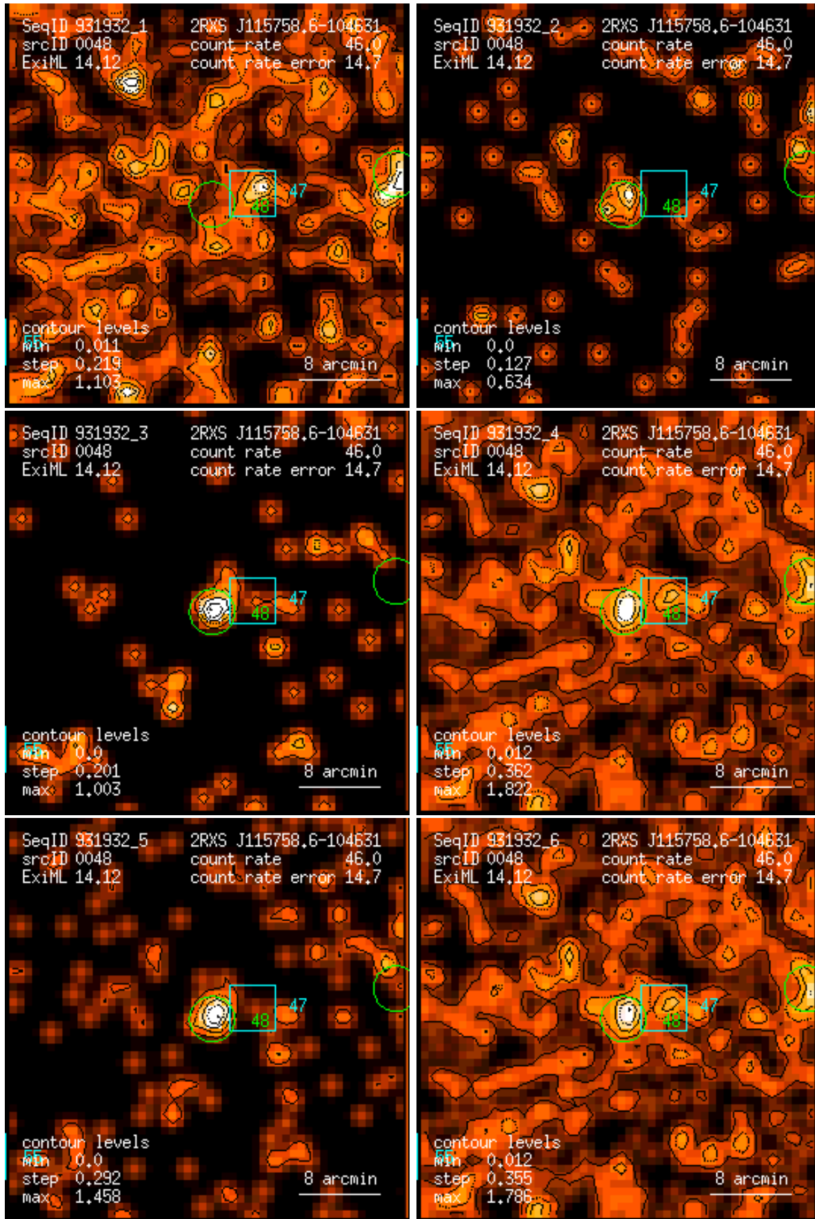
Figure 48: RASS 931932: detection 0048: band rate images, Gaussian filter: (1) PSPC channels 11 – 41, (2) 52 – 90, (3) 91 – 201, (4) 11 – 235, (5) 52 – 201, (6) 11 – 201. Broad band rates in counts/ks. Band rate contour levels in counts/ks/arcmin 2 .
