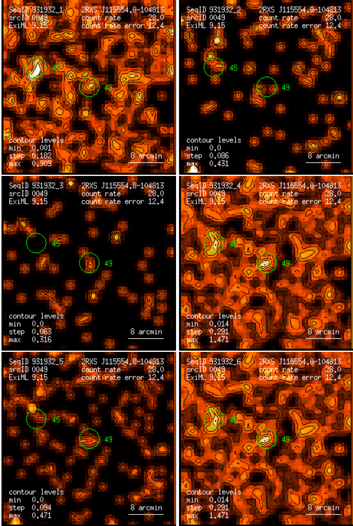
Figure 49: RASS 931932: detection 0049: band rate images, Gaussian filter: (1) PSPC channels 11 – 41, (2) 52 – 90, (3) 91 – 201, (4) 11 – 235, (5) 52 – 201, (6) 11 – 201. Broad band rates in counts/ks. Band rate contour levels in counts/ks/arcmin 2 .
