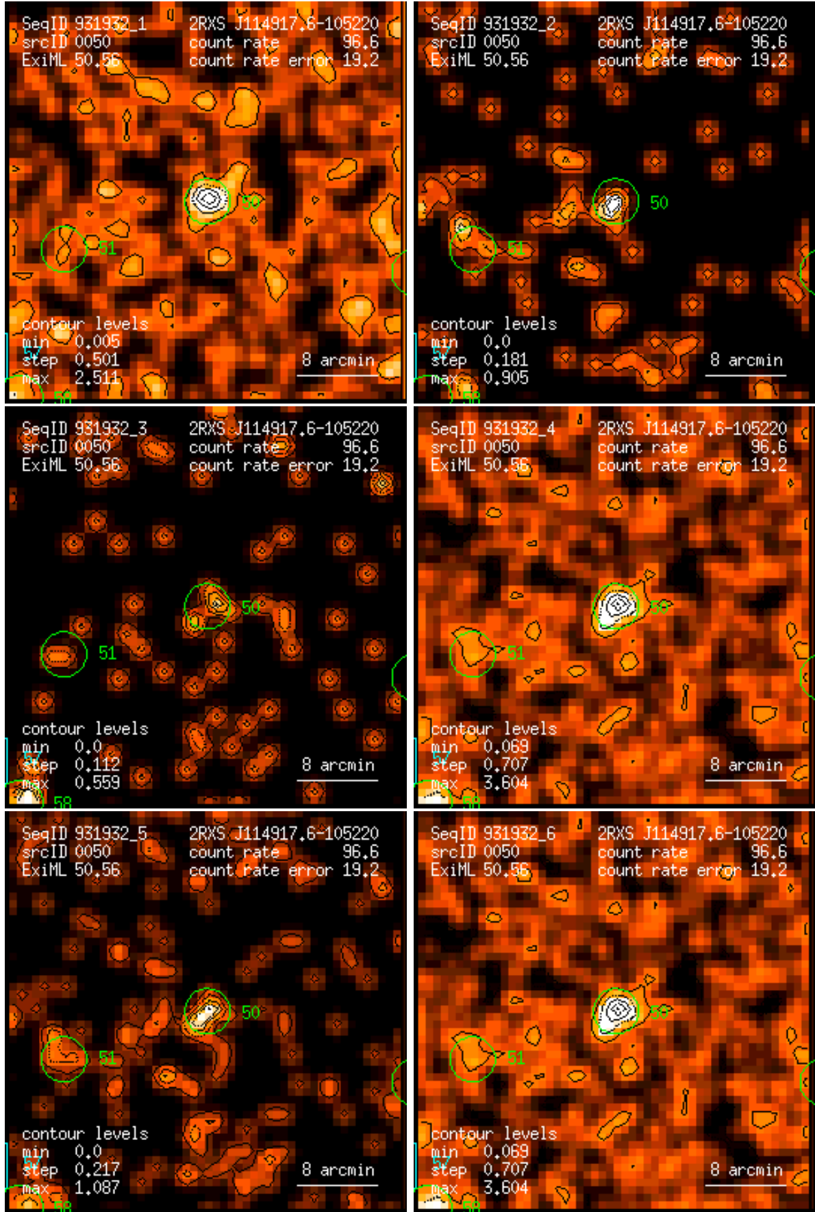
Figure 50: RASS 931932: detection 0050: band rate images, Gaussian filter: (1) PSPC channels 11 – 41, (2) 52 – 90, (3) 91 – 201, (4) 11 – 235, (5) 52 – 201, (6) 11 – 201. Broad band rates in counts/ks. Band rate contour levels in counts/ks/arcmin 2 .
