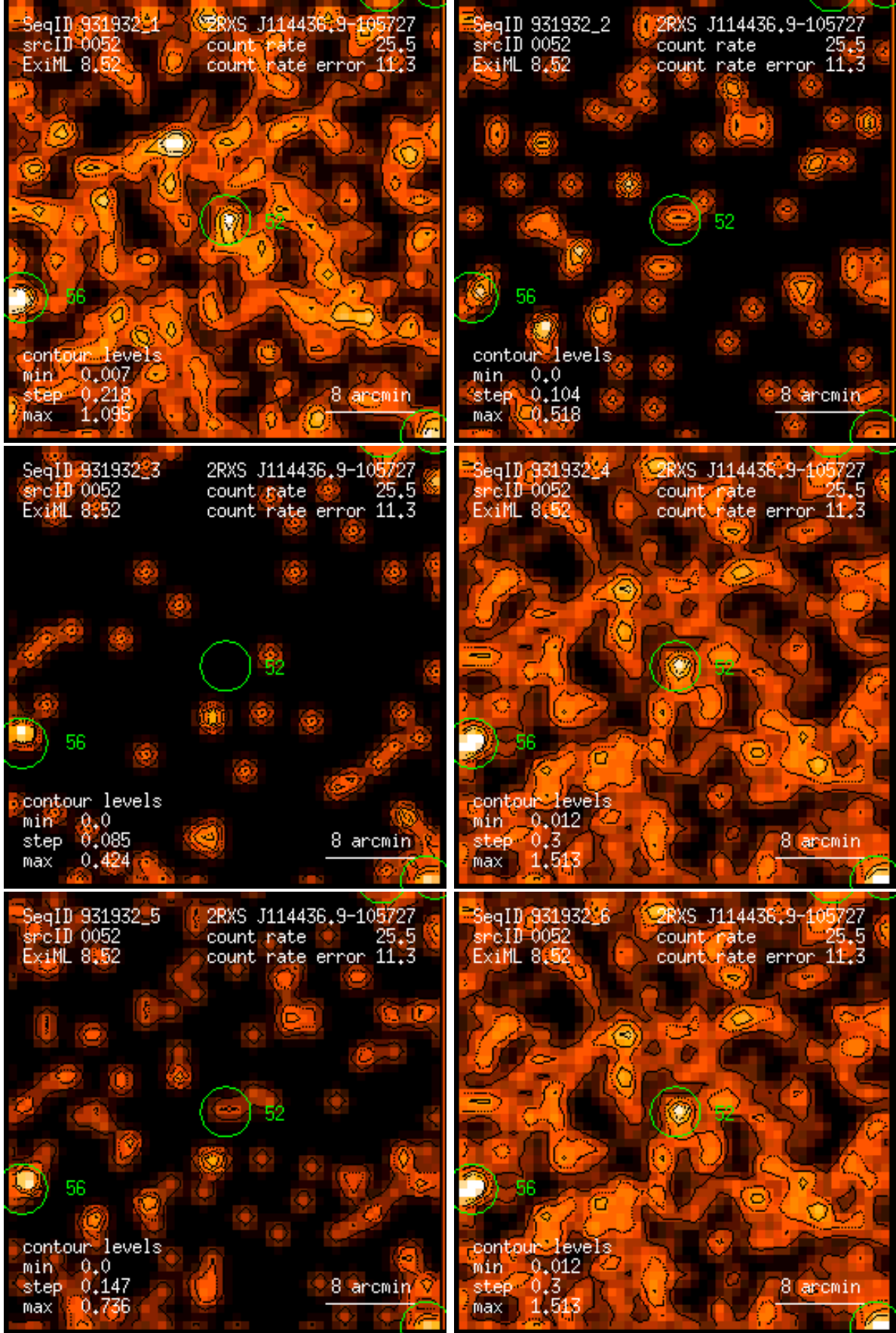
Figure 52: RASS 931932: detection 0052: band rate images, Gaussian filter: (1) PSPC channels 11 – 41, (2) 52 – 90, (3) 91 – 201, (4) 11 – 235, (5) 52 – 201, (6) 11 – 201. Broad band rates in counts/ks. Band rate contour levels in counts/ks/arcmin 2 .
