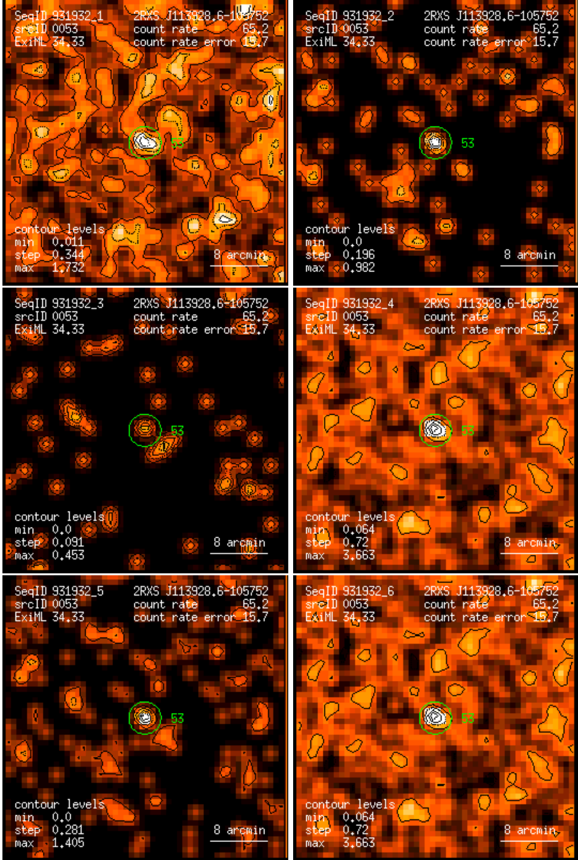
Figure 53: RASS 931932: detection 0053: band rate images, Gaussian filter: (1) PSPC channels 11 – 41, (2) 52 – 90, (3) 91 – 201, (4) 11 – 235, (5) 52 – 201, (6) 11 – 201. Broad band rates in counts/ks. Band rate contour levels in counts/ks/arcmin 2 .
