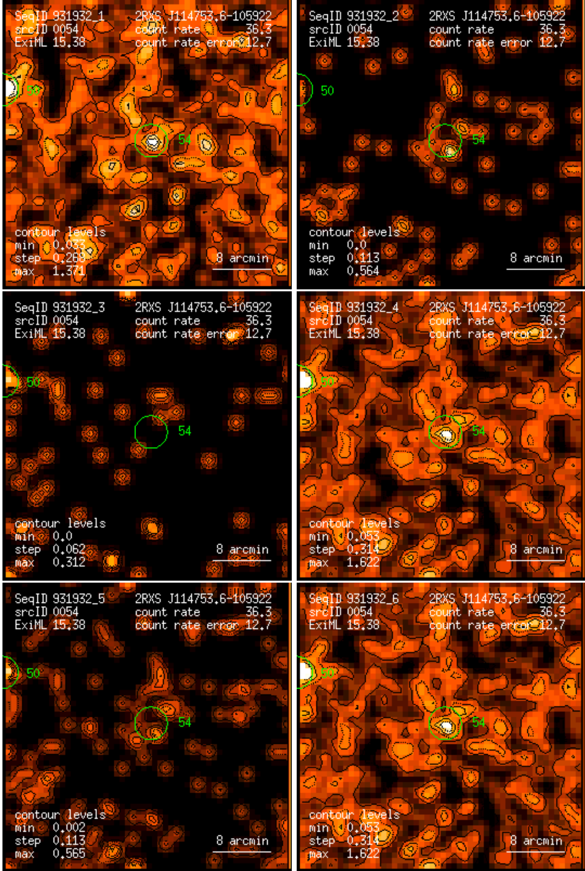
Figure 54: RASS 931932: detection 0054: band rate images, Gaussian filter: (1) PSPC channels 11 – 41, (2) 52 – 90, (3) 91 – 201, (4) 11 – 235, (5) 52 – 201, (6) 11 – 201. Broad band rates in counts/ks. Band rate contour levels in counts/ks/arcmin 2 .
