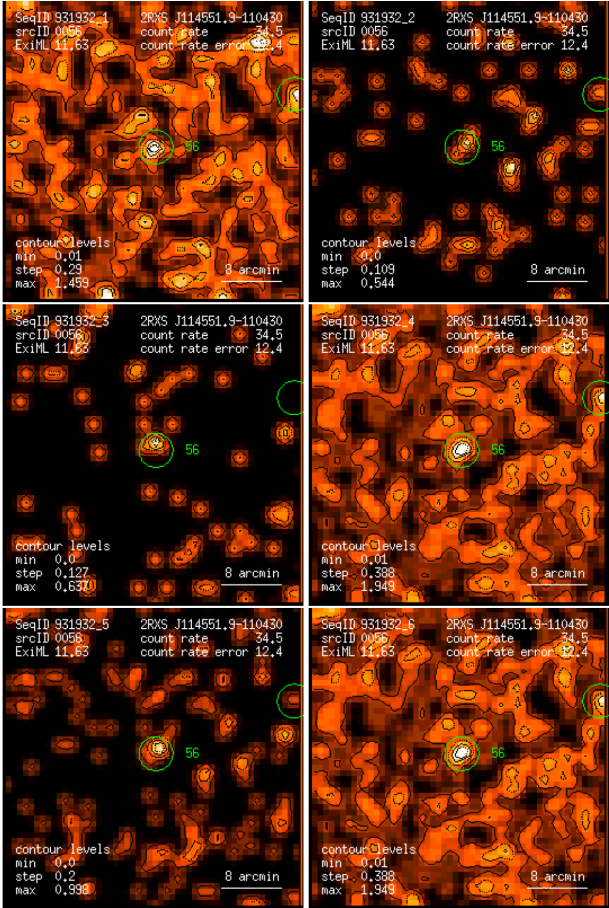
Figure 56: RASS 931932: detection 0056: band rate images, Gaussian filter: (1) PSPC channels 11 – 41, (2) 52 – 90, (3) 91 – 201, (4) 11 – 235, (5) 52 – 201, (6) 11 – 201. Broad band rates in counts/ks. Band rate contour levels in counts/ks/arcmin 2 .
