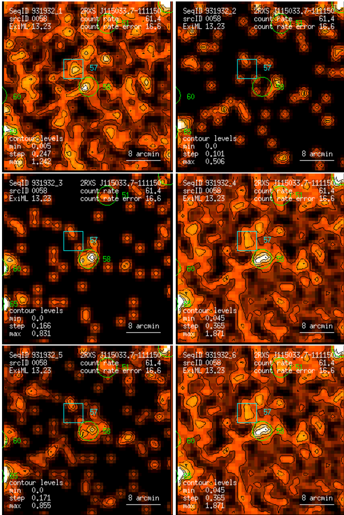
Figure 58: RASS 931932: detection 0058: band rate images, Gaussian filter: (1) PSPC channels 11 – 41, (2) 52 – 90, (3) 91 – 201, (4) 11 – 235, (5) 52 – 201, (6) 11 – 201. Broad band rates in counts/ks. Band rate contour levels in counts/ks/arcmin 2 .
