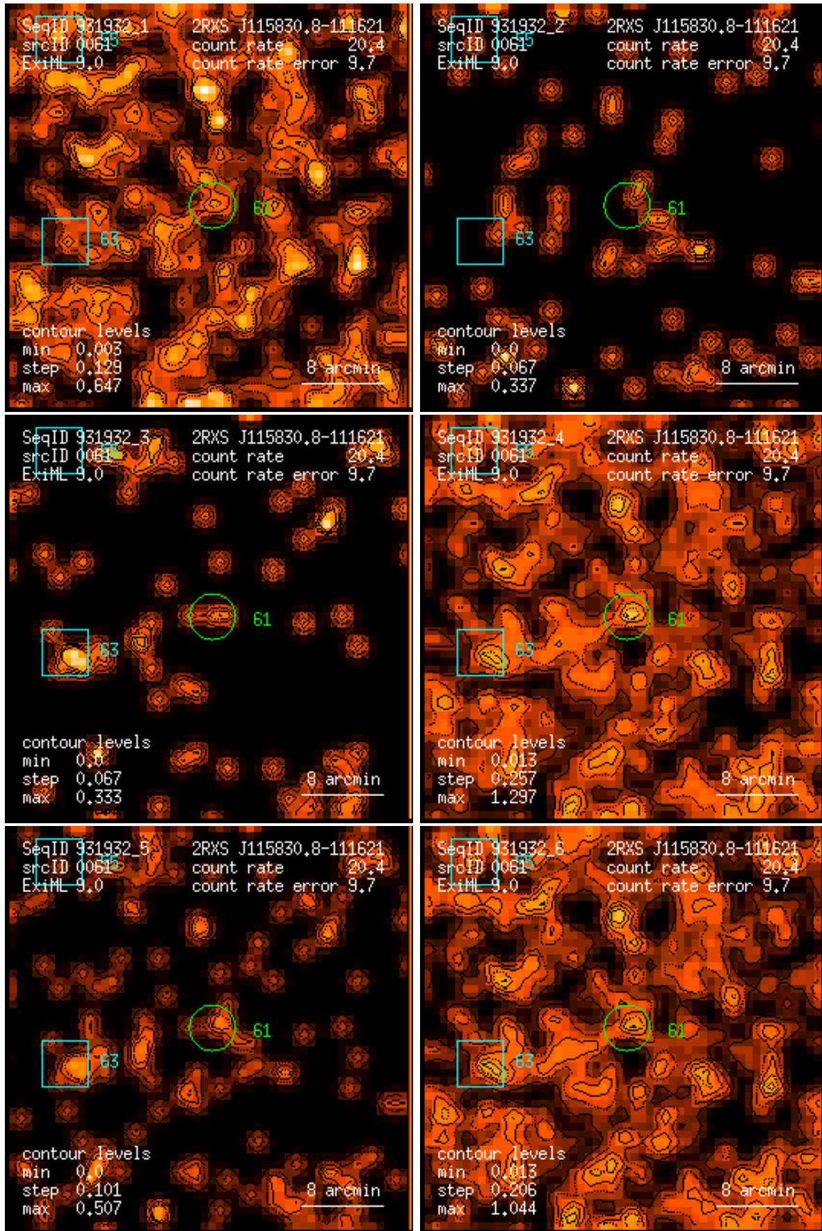
Figure 61: RASS 931932: detection 0061: band rate images, Gaussian filter: (1) PSPC channels 11 – 41, (2) 52 – 90, (3) 91 – 201, (4) 11 – 235, (5) 52 – 201, (6) 11 – 201. Broad band rates in counts/ks. Band rate contour levels in counts/ks/arcmin 2 .
