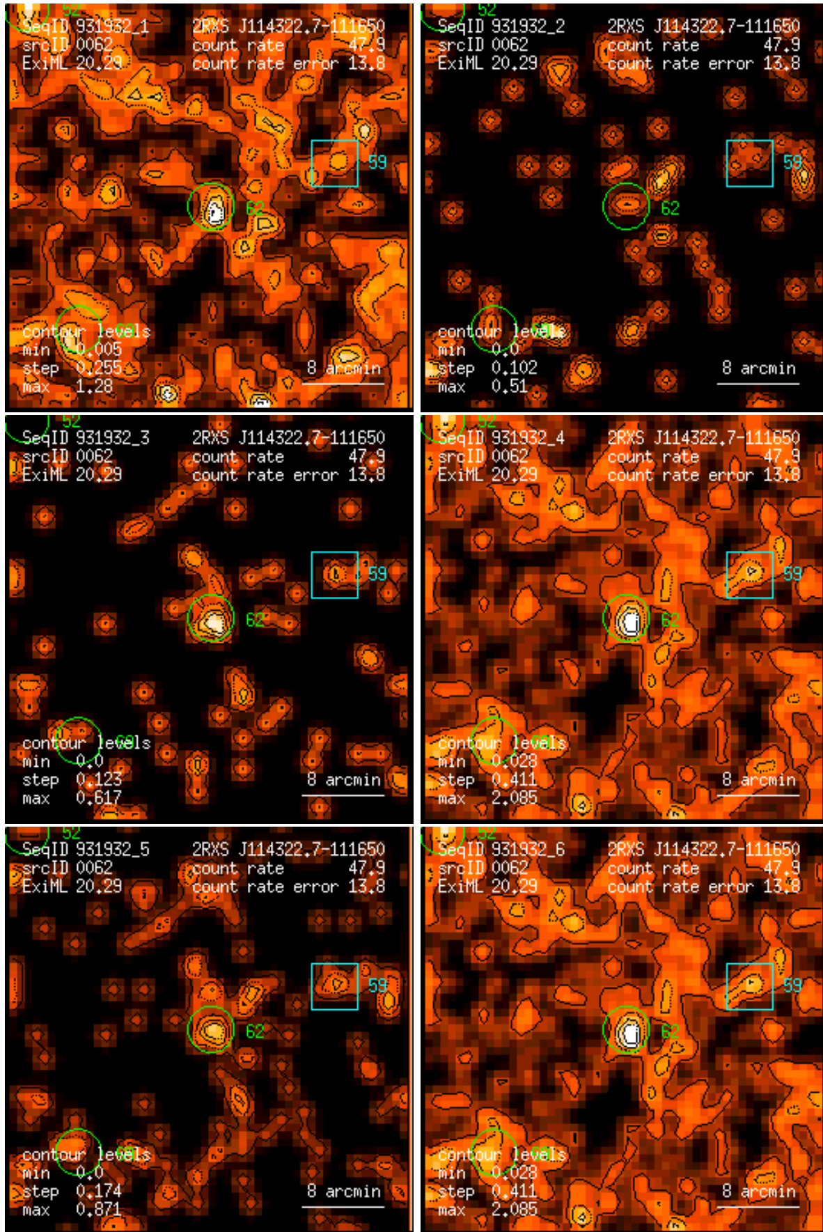
Figure 62: RASS 931932: detection 0062: band rate images, Gaussian filter: (1) PSPC channels 11 – 41, (2) 52 – 90, (3) 91 – 201, (4) 11 – 235, (5) 52 – 201, (6) 11 – 201. Broad band rates in counts/ks. Band rate contour levels in counts/ks/arcmin 2 .
