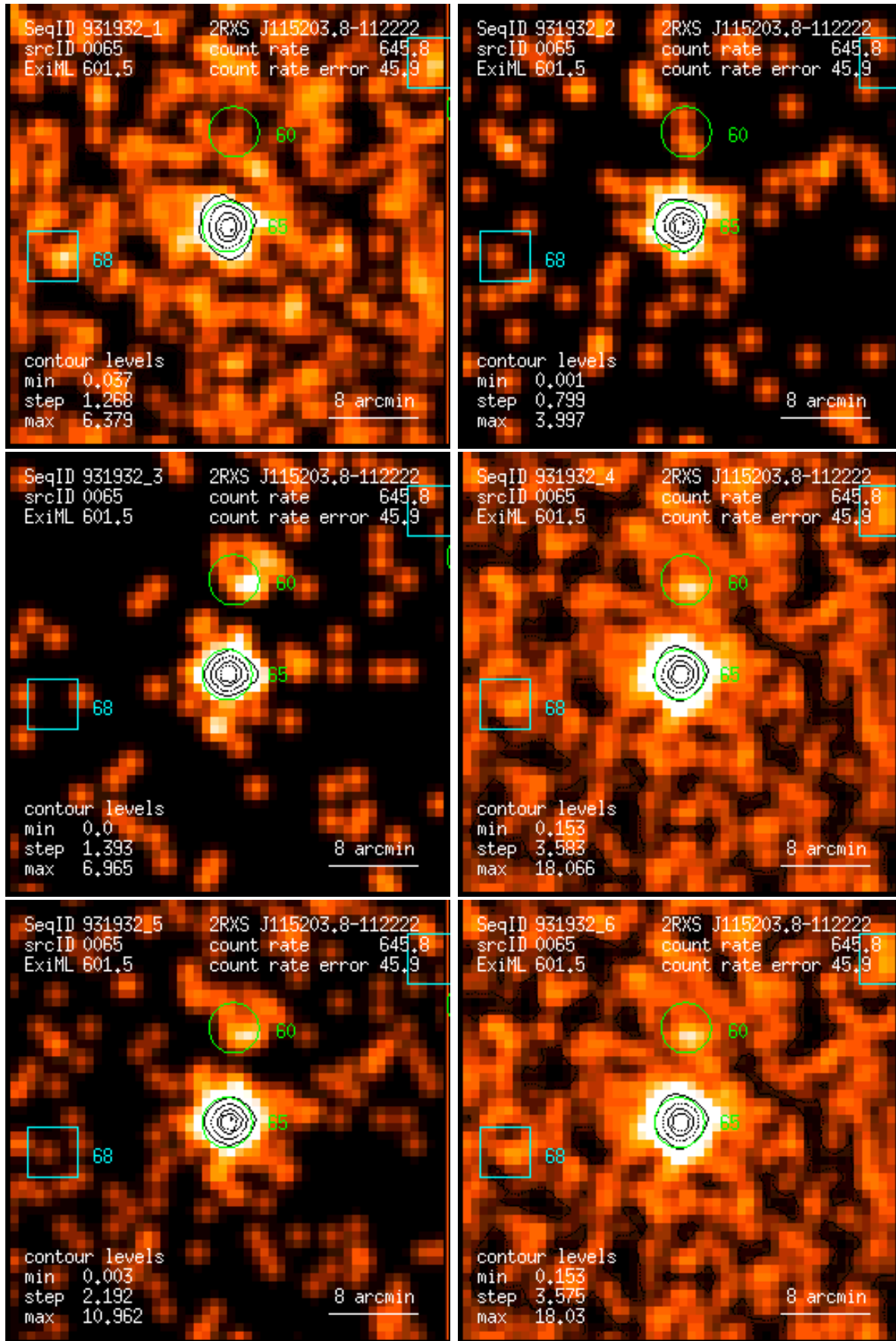
Figure 65: RASS 931932: detection 0065: band rate images, Gaussian filter: (1) PSPC channels 11 – 41, (2) 52 – 90, (3) 91 – 201, (4) 11 – 235, (5) 52 – 201, (6) 11 – 201. Broad band rates in counts/ks. Band rate contour levels in counts/ks/arcmin 2 .
