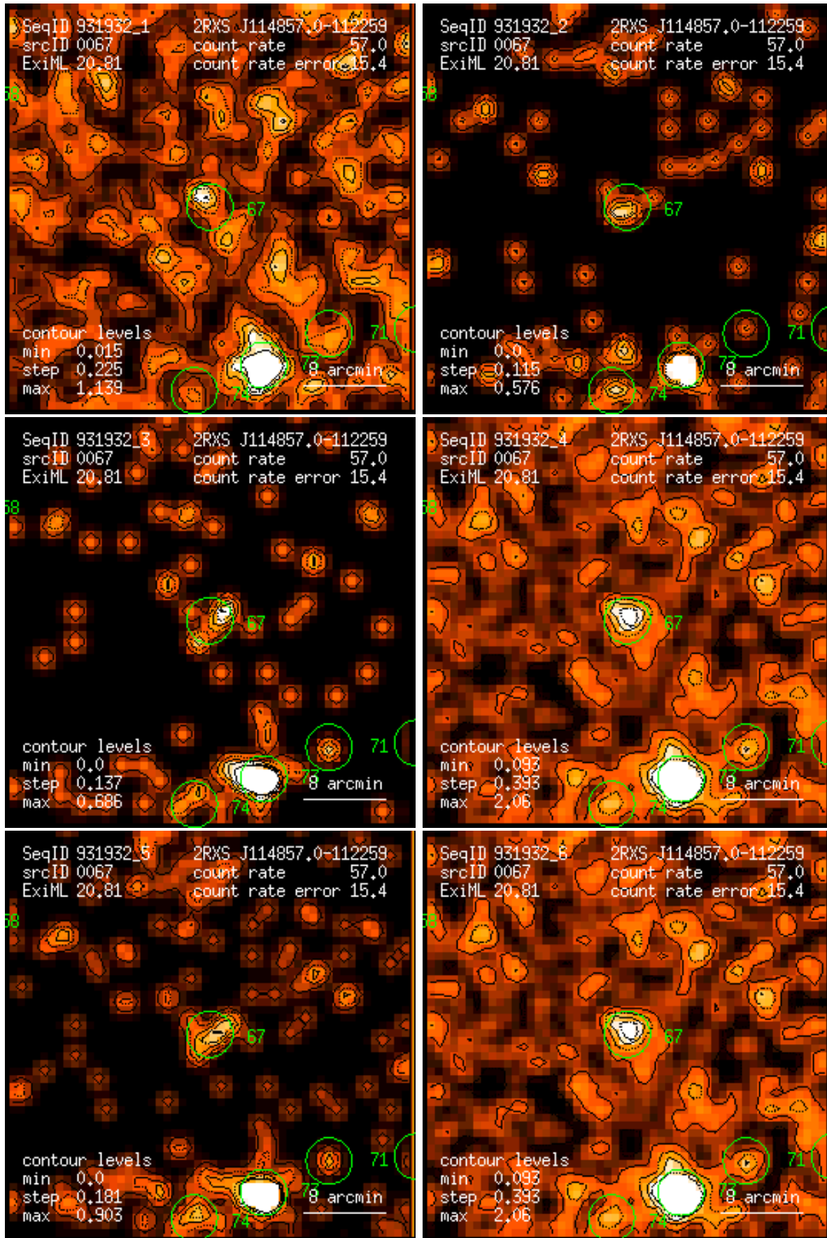
Figure 67: RASS 931932: detection 0067: band rate images, Gaussian filter: (1) PSPC channels 11 – 41, (2) 52 – 90, (3) 91 – 201, (4) 11 – 235, (5) 52 – 201, (6) 11 – 201. Broad band rates in counts/ks. Band rate contour levels in counts/ks/arcmin 2 .
