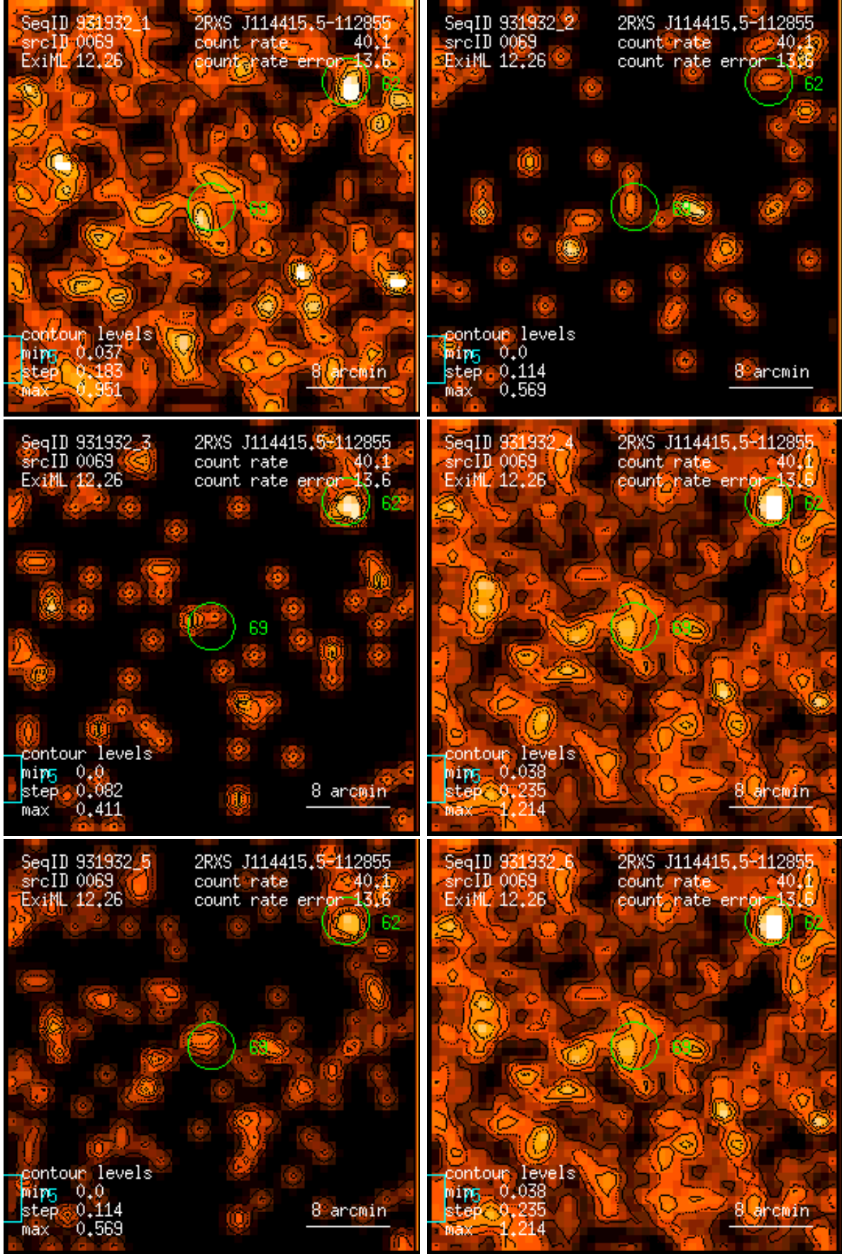
Figure 69: RASS 931932: detection 0069: band rate images, Gaussian filter: (1) PSPC channels 11 – 41, (2) 52 – 90, (3) 91 – 201, (4) 11 – 235, (5) 52 – 201, (6) 11 – 201. Broad band rates in counts/ks. Band rate contour levels in counts/ks/arcmin 2 .
