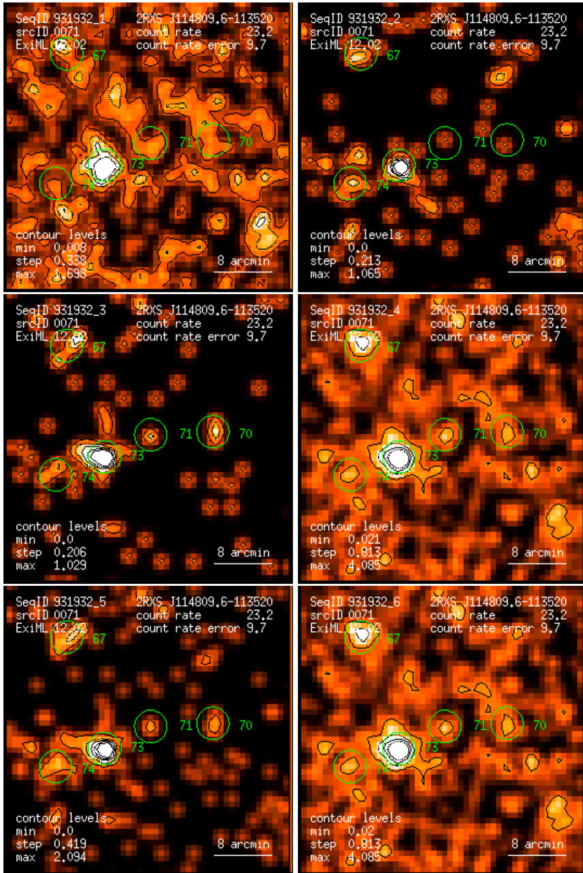
Figure 71: RASS 931932: detection 0071: band rate images, Gaussian filter: (1) PSPC channels 11 – 41, (2) 52 – 90, (3) 91 – 201, (4) 11 – 235, (5) 52 – 201, (6) 11 – 201. Broad band rates in counts/ks. Band rate contour levels in counts/ks/arcmin 2 .
