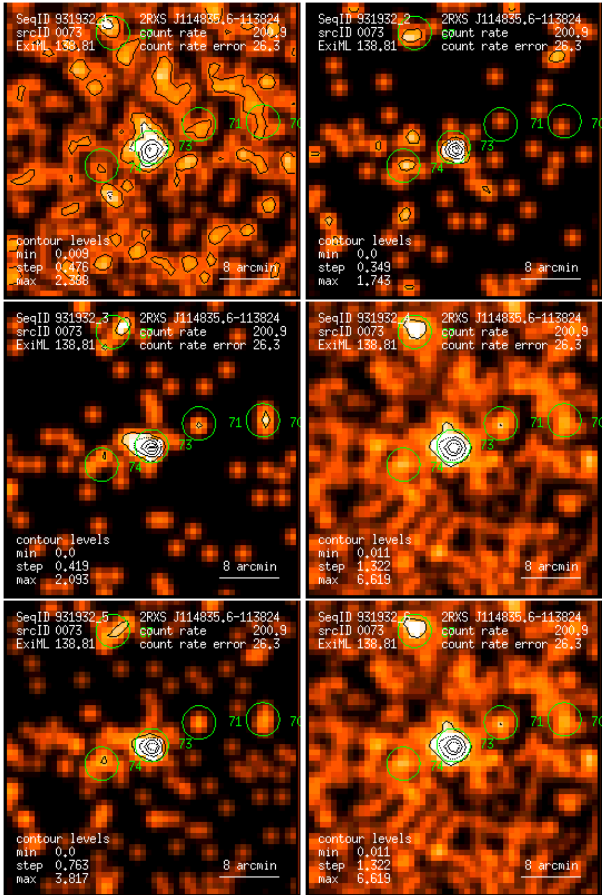
Figure 73: RASS 931932: detection 0073: band rate images, Gaussian filter: (1) PSPC channels 11 – 41, (2) 52 – 90, (3) 91 – 201, (4) 11 – 235, (5) 52 – 201, (6) 11 – 201. Broad band rates in counts/ks. Band rate contour levels in counts/ks/arcmin 2 .
