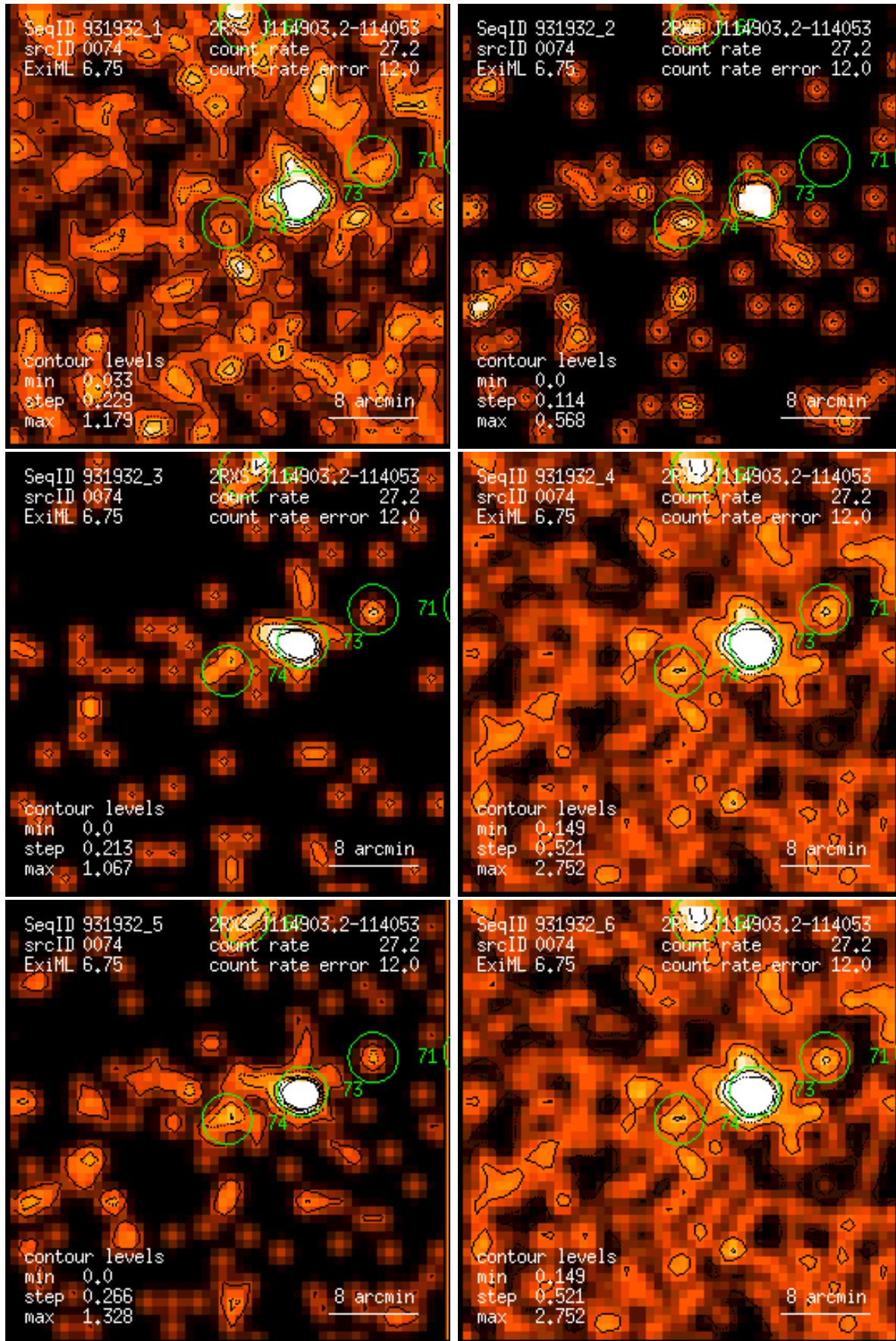
Figure 74: RASS 931932: detection 0074: band rate images, Gaussian filter: (1) PSPC channels 11 – 41, (2) 52 – 90, (3) 91 – 201, (4) 11 – 235, (5) 52 – 201, (6) 11 – 201. Broad band rates in counts/ks. Band rate contour levels in counts/ks/arcmin 2 .
