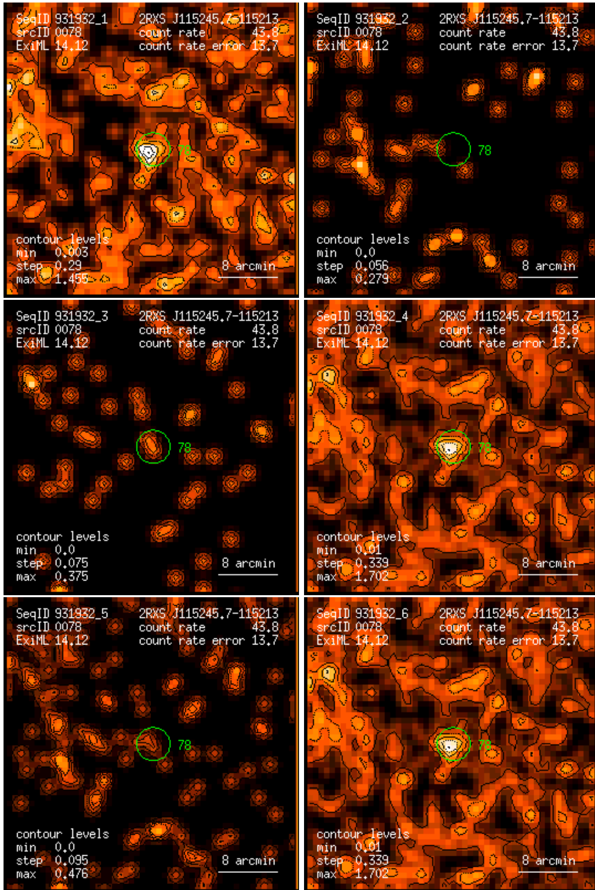
Figure 78: RASS 931932: detection 0078: band rate images, Gaussian filter: (1) PSPC channels 11 – 41, (2) 52 – 90, (3) 91 – 201, (4) 11 – 235, (5) 52 – 201, (6) 11 – 201. Broad band rates in counts/ks. Band rate contour levels in counts/ks/arcmin 2 .
