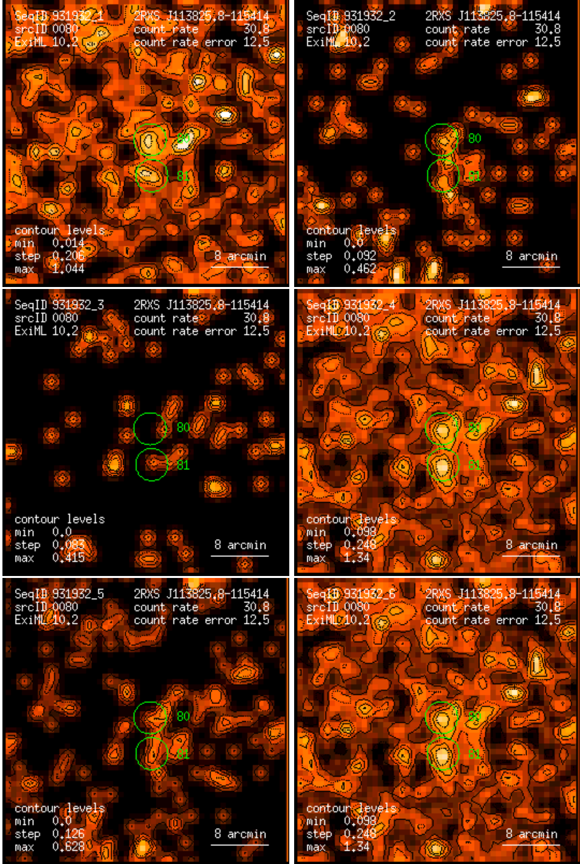
Figure 80: RASS 931932: detection 0080: band rate images, Gaussian filter: (1) PSPC channels 11 – 41, (2) 52 – 90, (3) 91 – 201, (4) 11 – 235, (5) 52 – 201, (6) 11 – 201. Broad band rates in counts/ks. Band rate contour levels in counts/ks/arcmin 2 .
