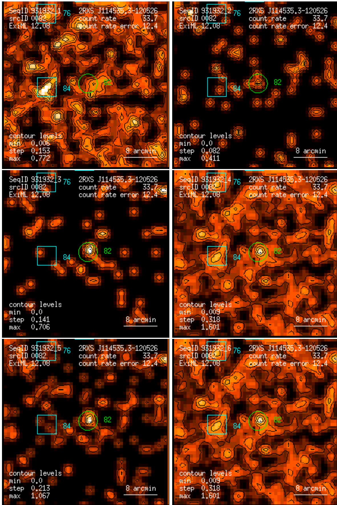
Figure 82: RASS 931932: detection 0082: band rate images, Gaussian filter: (1) PSPC channels 11 – 41, (2) 52 – 90, (3) 91 – 201, (4) 11 – 235, (5) 52 – 201, (6) 11 – 201. Broad band rates in counts/ks. Band rate contour levels in counts/ks/arcmin 2 .
