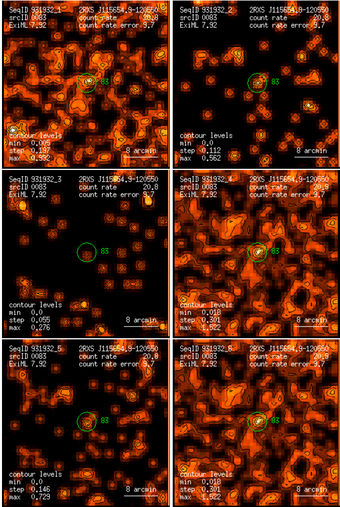
Figure 83: RASS 931932: detection 0083: band rate images, Gaussian filter: (1) PSPC channels 11 – 41, (2) 52 – 90, (3) 91 – 201, (4) 11 – 235, (5) 52 – 201, (6) 11 – 201. Broad band rates in counts/ks. Band rate contour levels in counts/ks/arcmin 2 .
