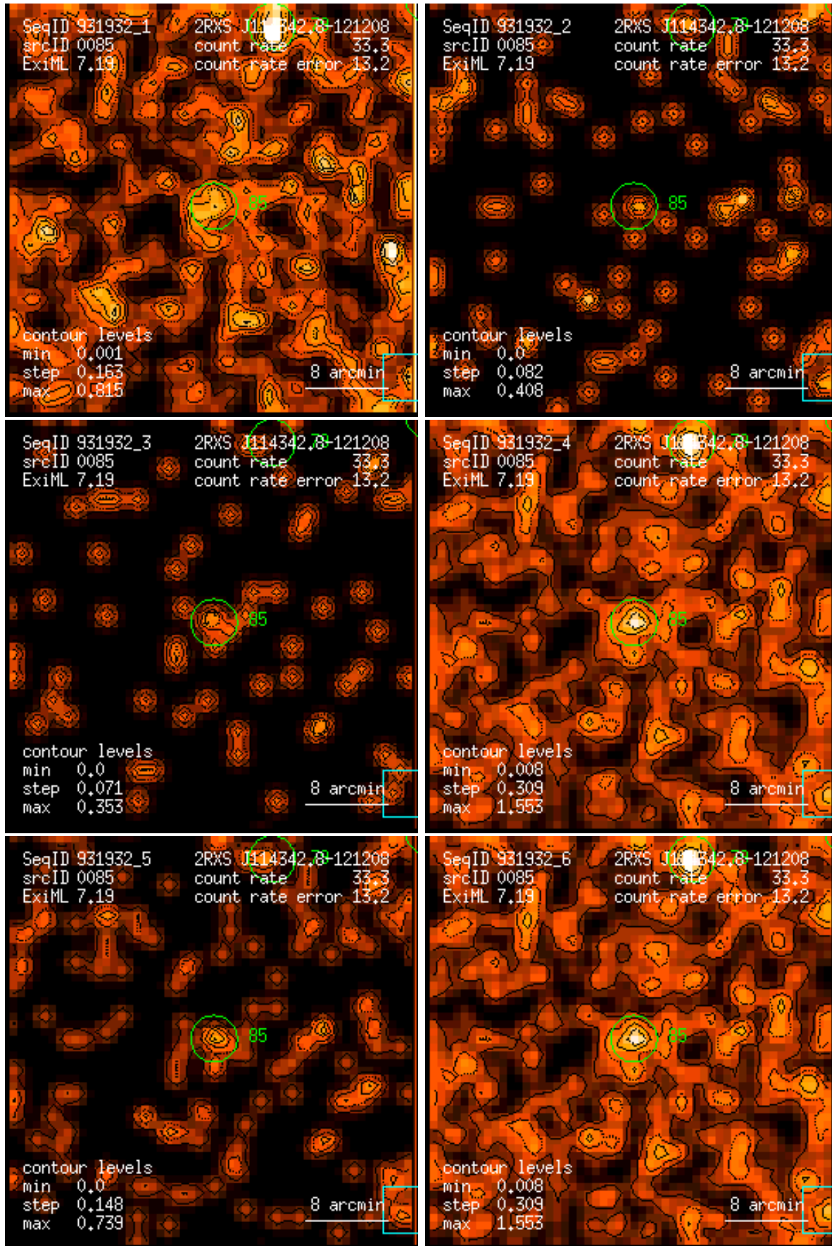
Figure 85: RASS 931932: detection 0085: band rate images, Gaussian filter: (1) PSPC channels 11 – 41, (2) 52 – 90, (3) 91 – 201, (4) 11 – 235, (5) 52 – 201, (6) 11 – 201. Broad band rates in counts/ks. Band rate contour levels in counts/ks/arcmin 2 .
