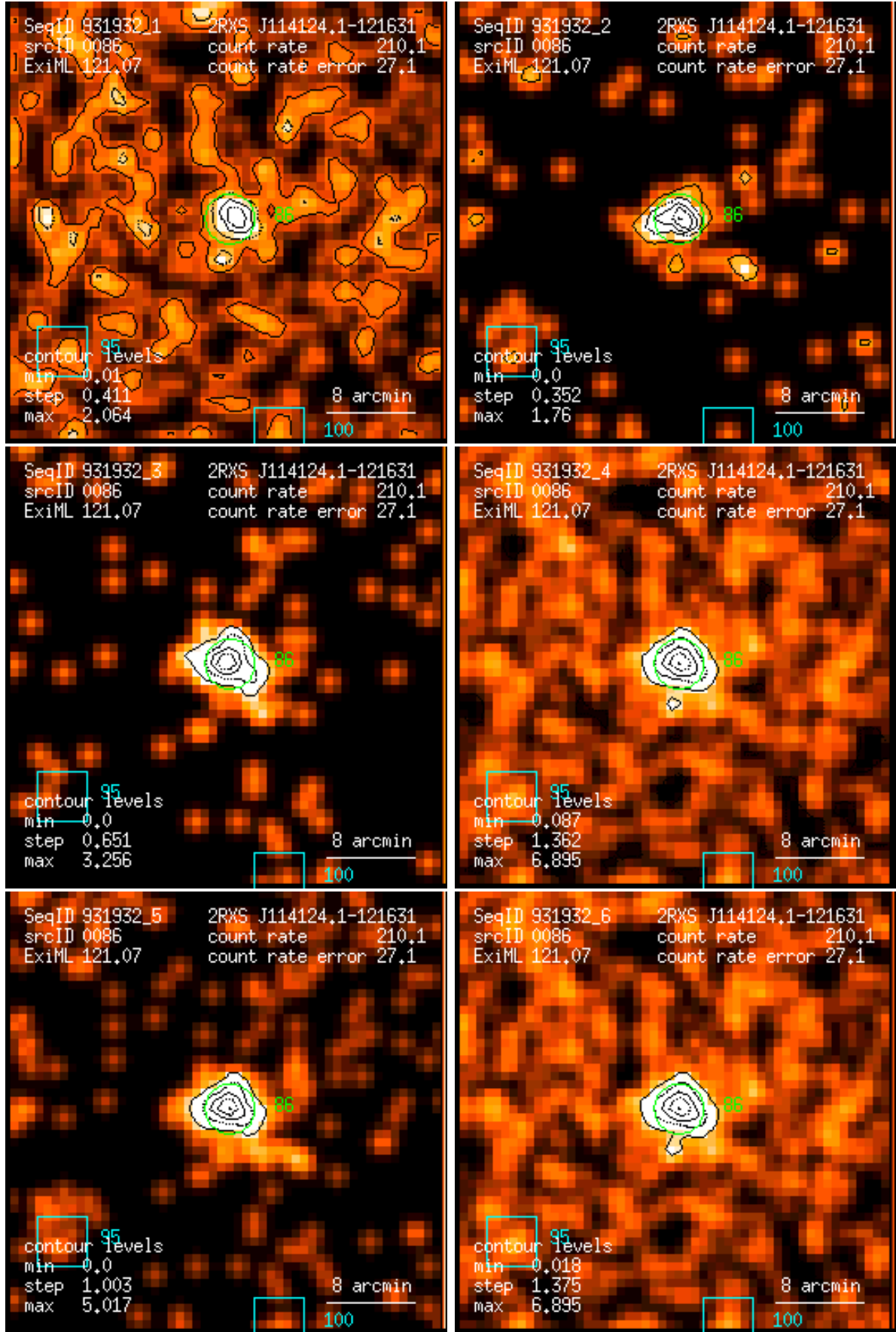
Figure 86: RASS 931932: detection 0086: band rate images, Gaussian filter: (1) PSPC channels 11 – 41, (2) 52 – 90, (3) 91 – 201, (4) 11 – 235, (5) 52 – 201, (6) 11 – 201. Broad band rates in counts/ks. Band rate contour levels in counts/ks/arcmin 2 .
