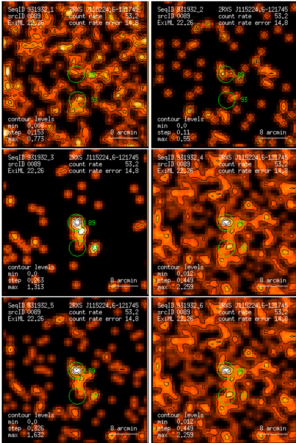
Figure 89: RASS 931932: detection 0089: band rate images, Gaussian filter: (1) PSPC channels 11 – 41, (2) 52 – 90, (3) 91 – 201, (4) 11 – 235, (5) 52 – 201, (6) 11 – 201. Broad band rates in counts/ks. Band rate contour levels in counts/ks/arcmin 2 .
