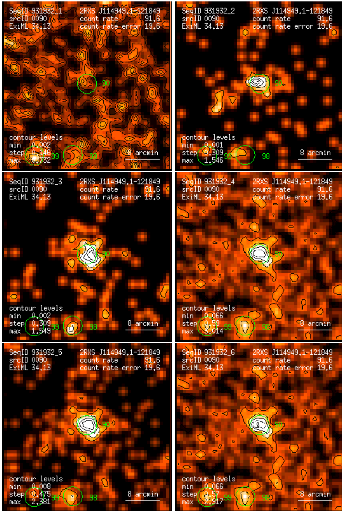
Figure 90: RASS 931932: detection 0090: band rate images, Gaussian filter: (1) PSPC channels 11 – 41, (2) 52 – 90, (3) 91 – 201, (4) 11 – 235, (5) 52 – 201, (6) 11 – 201. Broad band rates in counts/ks. Band rate contour levels in counts/ks/arcmin 2 .
