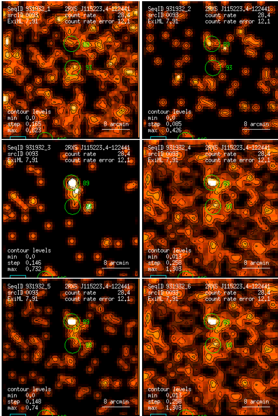
Figure 93: RASS 931932: detection 0093: band rate images, Gaussian filter: (1) PSPC channels 11 – 41, (2) 52 – 90, (3) 91 – 201, (4) 11 – 235, (5) 52 – 201, (6) 11 – 201. Broad band rates in counts/ks. Band rate contour levels in counts/ks/arcmin 2 .
