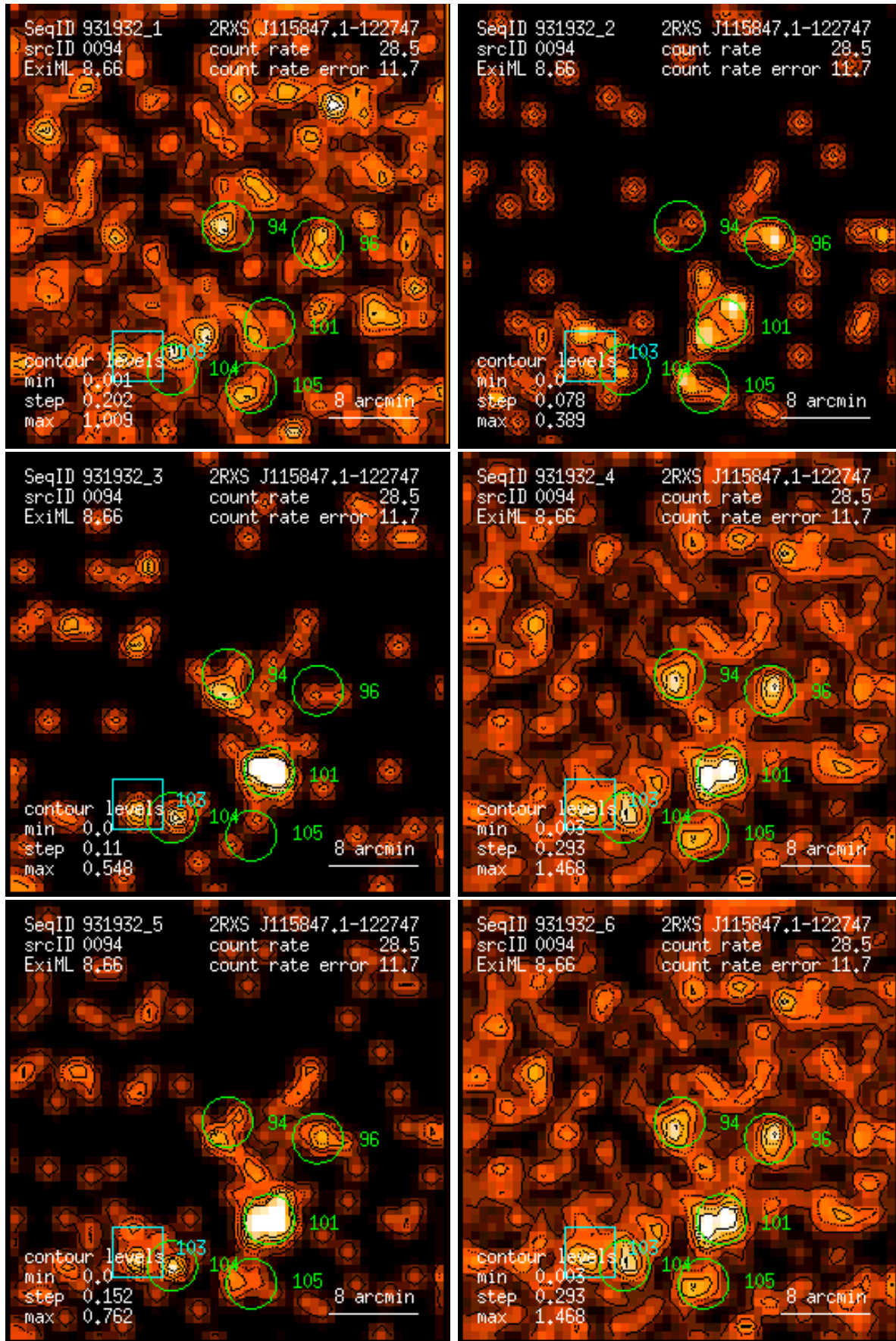
Figure 94: RASS 931932: detection 0094: band rate images, Gaussian filter: (1) PSPC channels 11 – 41, (2) 52 – 90, (3) 91 – 201, (4) 11 – 235, (5) 52 – 201, (6) 11 – 201. Broad band rates in counts/ks. Band rate contour levels in counts/ks/arcmin 2 .
