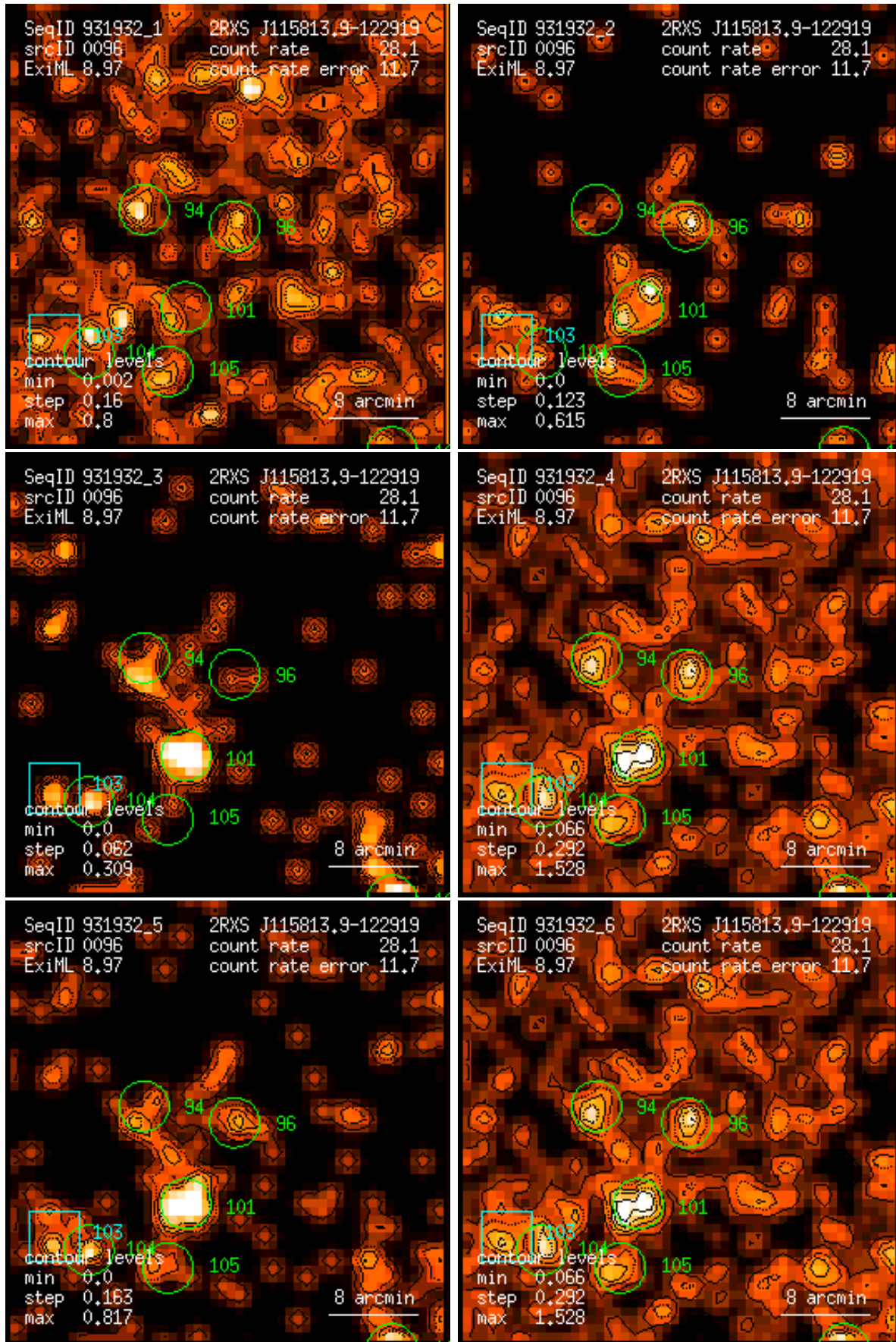
Figure 96: RASS 931932: detection 0096: band rate images, Gaussian filter: (1) PSPC channels 11 – 41, (2) 52 – 90, (3) 91 – 201, (4) 11 – 235, (5) 52 – 201, (6) 11 – 201. Broad band rates in counts/ks. Band rate contour levels in counts/ks/arcmin 2 .
