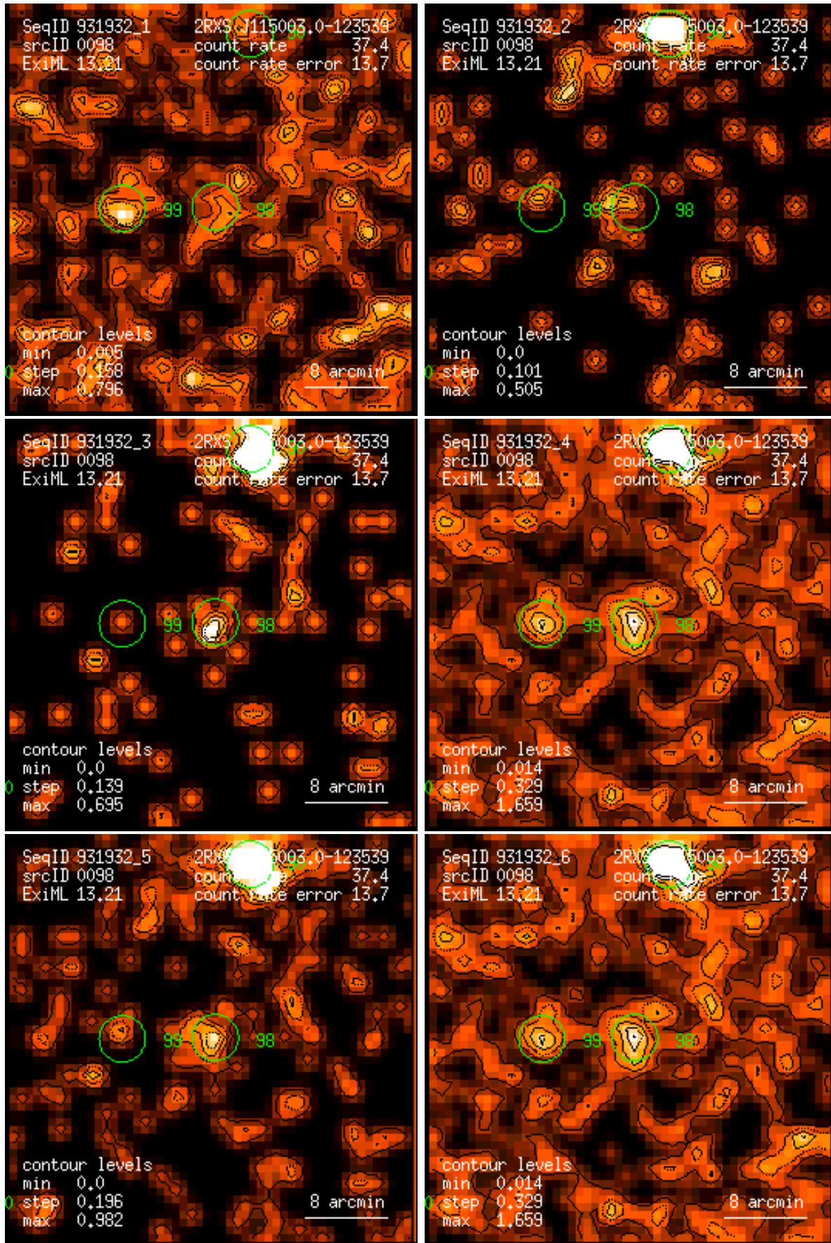
Figure 98: RASS 931932: detection 0098: band rate images, Gaussian filter: (1) PSPC channels 11 – 41, (2) 52 – 90, (3) 91 – 201, (4) 11 – 235, (5) 52 – 201, (6) 11 – 201. Broad band rates in counts/ks. Band rate contour levels in counts/ks/arcmin 2 .
