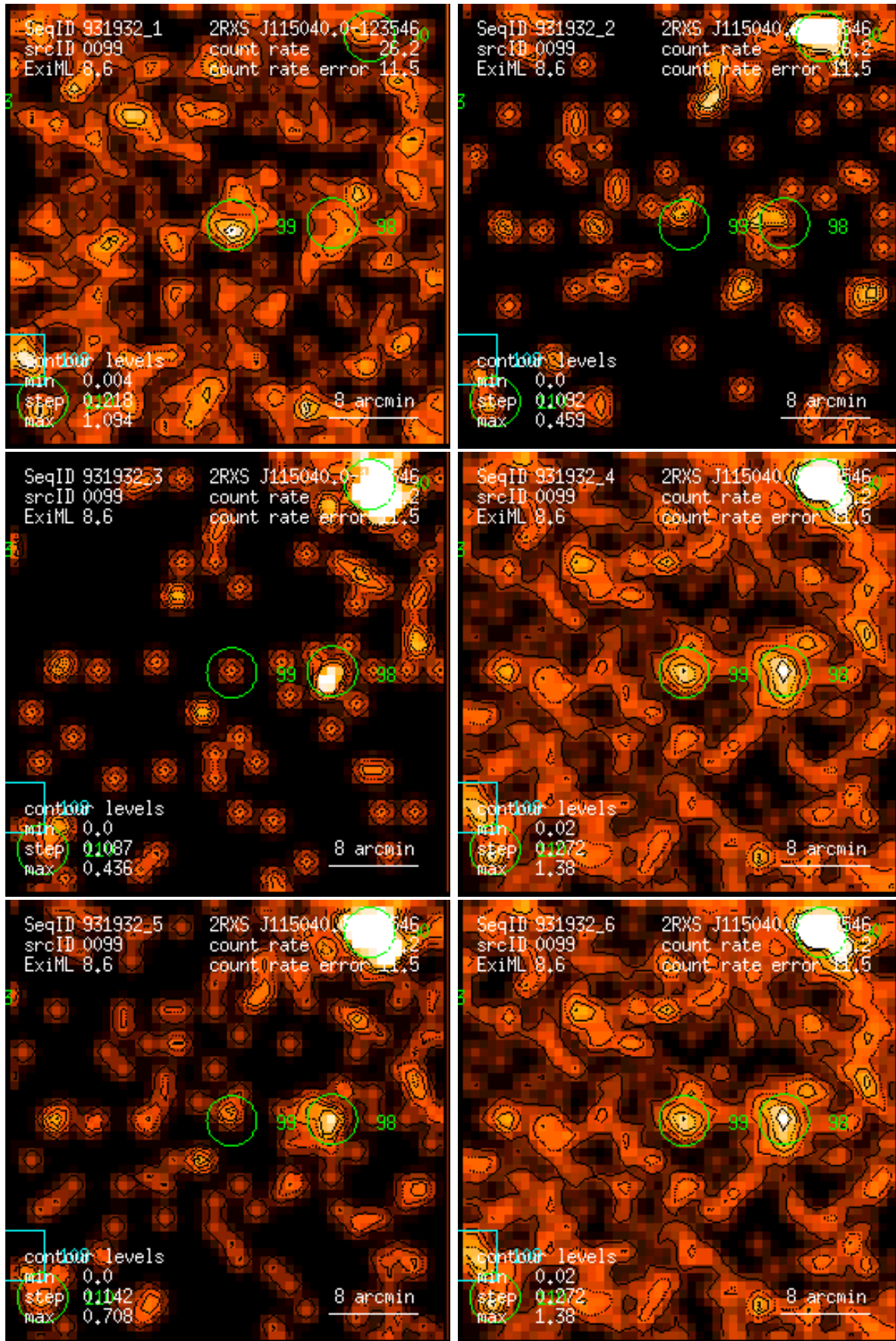
Figure 99: RASS 931932: detection 0099: band rate images, Gaussian filter: (1) PSPC channels 11 – 41, (2) 52 – 90, (3) 91 – 201, (4) 11 – 235, (5) 52 – 201, (6) 11 – 201. Broad band rates in counts/ks. Band rate contour levels in counts/ks/arcmin 2 .
